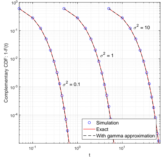
(b) The complementary CDF (CCDF) of \zeta_e .
