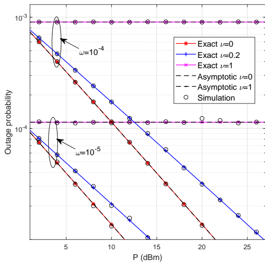
(a) The outage probability vs P .
