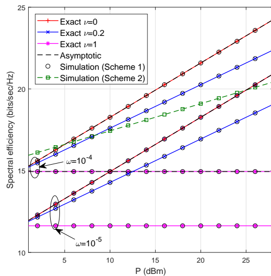
(b) The spectral efficiency vs P .
