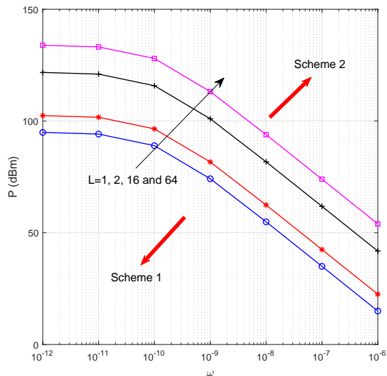
(b) The transmit power vs n of \sigma_i^2 = \omega P = 10^{-n} P .
