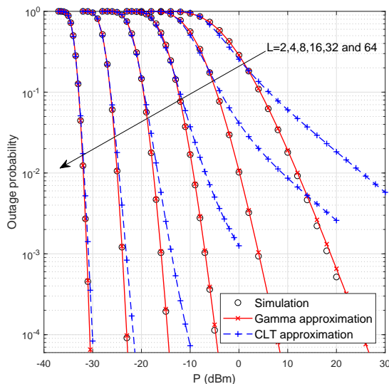
Fig. 5: The outage probability vs P when \sigma_i^2 = 10^{-4} .
