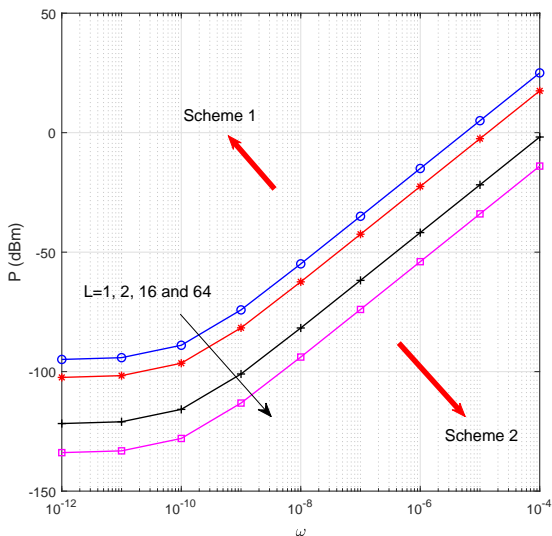
(a) The transmit power vs n of \sigma_i^2 = \omega = 10^{-n} .
