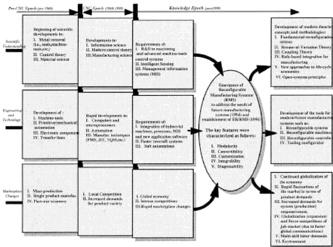
Fig. 3. The key role of reconfigurable manufacturing systems (RMS) in future manufacturing.
