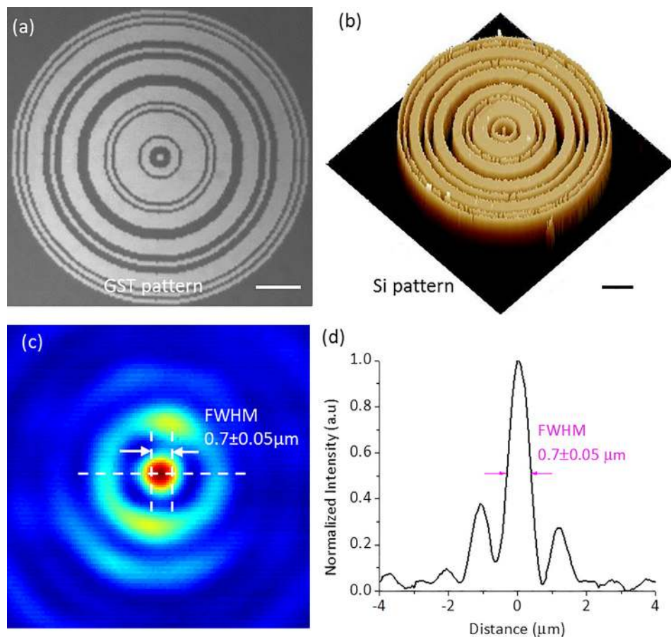
FIG. 4. Optical lithography of a sub-diffraction-limited focusing SOL in Si. (a) Reflection microscopy image of the SOL in GST (photomask). (b) AFM image of the two-step phase SOL etched in a Si wafer. The etch depth is 318 \pm 5 \text{ nm} . (c) Focused hotspot from the SOL at a wavelength of 1550 \text{ nm} . (d) The cross section of the SOL hotspot image shows that the FWHM size is 0.7 \mu\text{m} ( 0.45 \lambda ). The scale bar in (a) and (b) is 10 \mu\text{m} .
