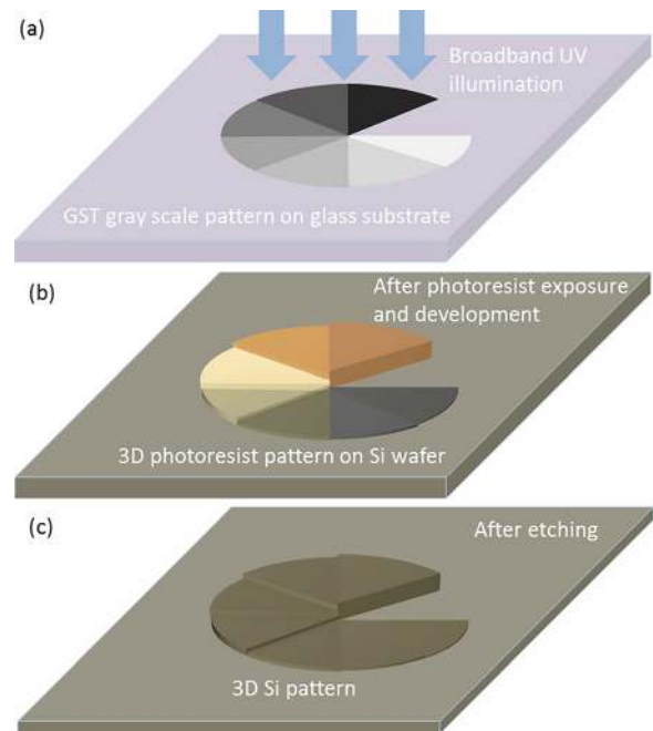
FIG. 1. Sketch of the 3D spiral phase plate fabrication process. (a) Grayscale photomask is prepared by direct optical writing in a GST thin film. (b) The photoresist is exposed and developed leaving a 3D photoresist structure on the substrate. (c) 3D silicon structure is obtained by uniform etching of the substrate and remaining photoresist.
