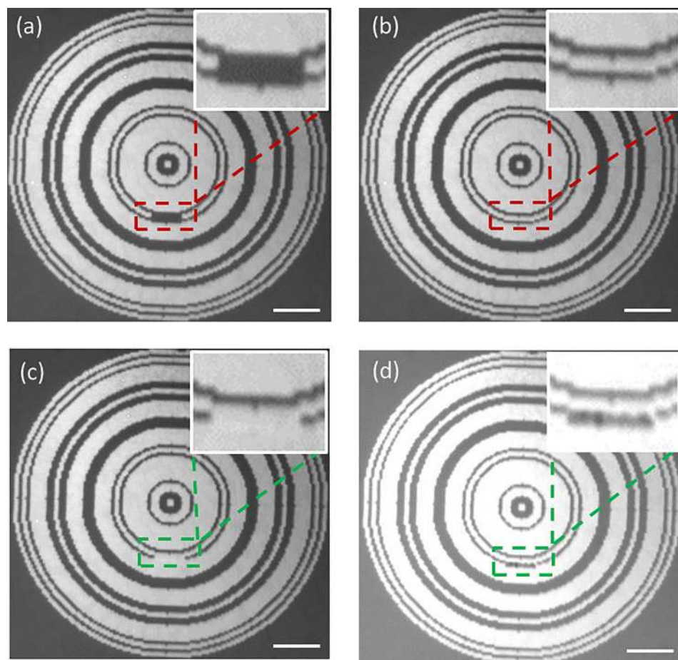
FIG. 3. Reconfiguration of a photomask on a GST film. (a) Optical micrograph of the written photomask with a deliberate defect: one crystallized line is missing. (b) The defect was subsequently corrected with another writing procedure crystallizing only the missing line. (c) Optical micrograph of a written photomask with a defect of an extra crystallized region ( 15 \times 1 pixels). (d) The defect was corrected by re-amorphization of the GST marks one by one. The scale bar is 10 \mu\text{m} .
