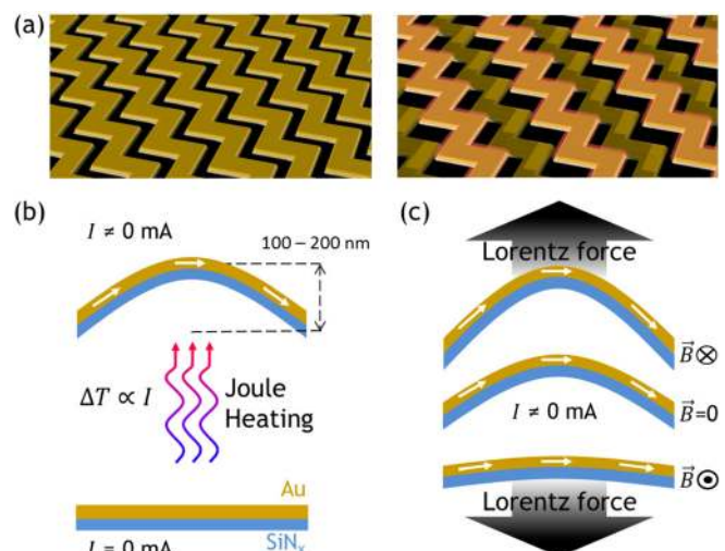
FIG. 1. Actuation mechanisms for electrically and magnetically reconfigurable metamaterial. (a) Artistic impression of the metamaterial's OFF state (left) and ON state (right). (b) Electrothermal tuning: Currents flowing in electrically connected bridges will produce Joule heating and bow the bilayered structure due to differential thermal expansion of gold (yellow) and silicon nitride (blue). (c) Magnetic tuning: Moving charges (current) in a static magnetic field will be subject to the Lorentz force that can be used to enhance or inhibit the electrothermal deformation.
