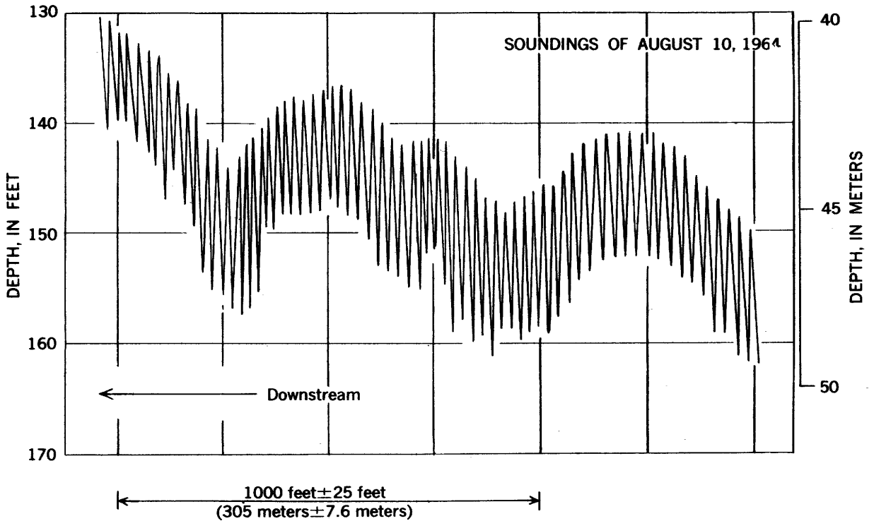
Figure 8.—Section of fathometer chart taken near midstream and crossing general location of measuring section, Amazon River at Óbidos.
