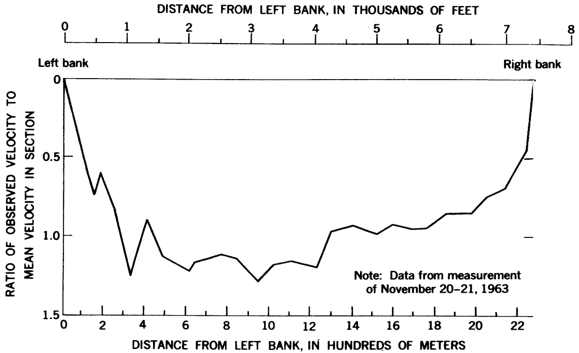
Figure 7.—Distribution of mean velocity in cross section, Amazon River at Óbidos.
