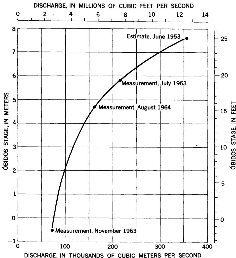
Figure 2.—Stage-discharge relation, Amazon River at Óbidos.
