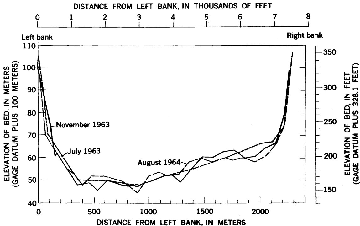
Figure 3.—Measured cross sections from three discharge measurements, Amazon River at Óbidos.
