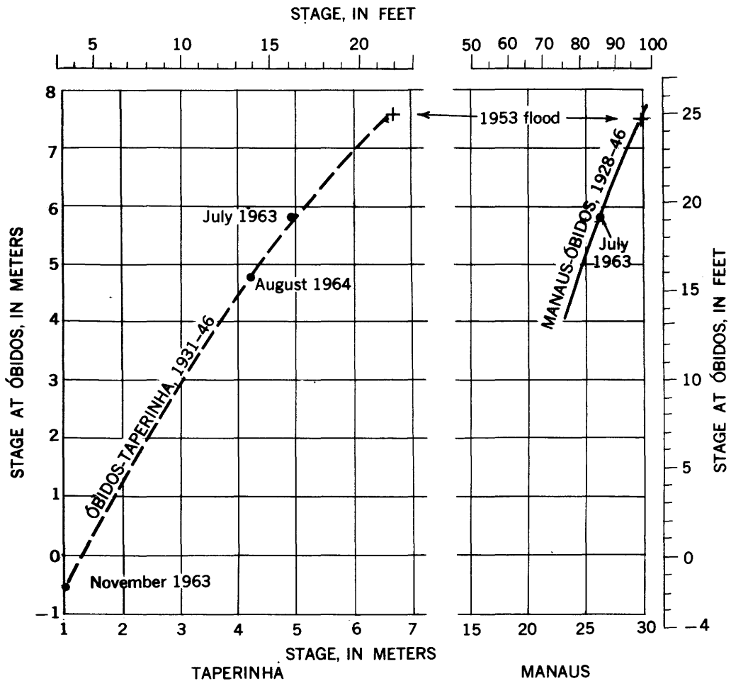
Figure 1.—Relation of concurrent readings on gages, Amazon River at Óbidos, Manaus, and Taperinha.
