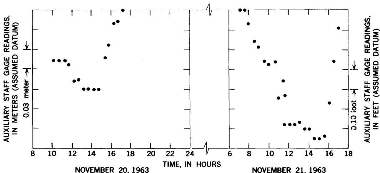
Figure 5.—Water level observations showing tidal effect at low flow, Amazon River at Óbidos. Auxiliary staff gage was moved at close of readings on November 20 and not set to same datum for readings of November 21.
