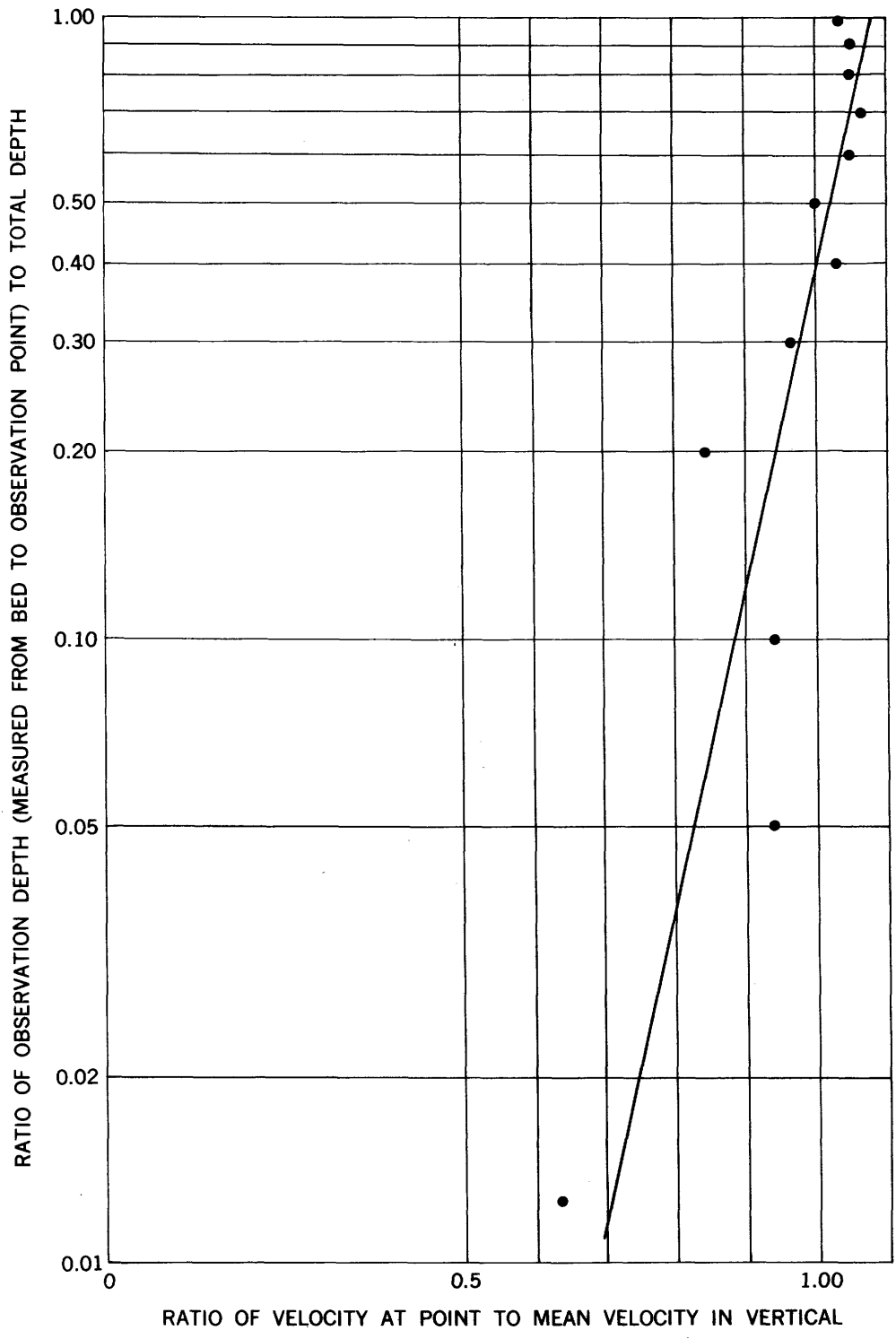
Figure 6.—Distribution of velocity in a selected vertical, Amazon River at Óbidos.
