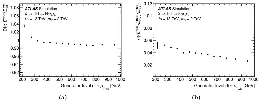
Figure 5. Energy (a) scale and (b) resolution of the di- \tau reconstruction as a function of the p_T of the di- \tau system at generator level, computed in simulated X \rightarrow HH \rightarrow bb\tau^+\tau^- events, where the resonance mass is set to 2 TeV and all \tau -leptons decay hadronically. The requirement of p_T > 300 GeV on the seeding jet truncates the reconstructed energy distribution and leads to a degradation of the energy scale for the lower values of the p_T of the di- \tau system. The vertical error bars only account for statistical uncertainties.
