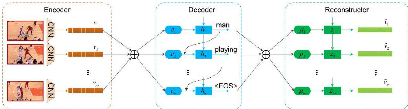
Figure 2. The proposed RecNet consists of three parts: the CNN-based encoder which extracts the semantic representations of the video frames, the LSTM-based decoder which generates natural language for visual content description, and the reconstructor which exploits the backward flow from caption to visual contents to reproduce the frame representations.
