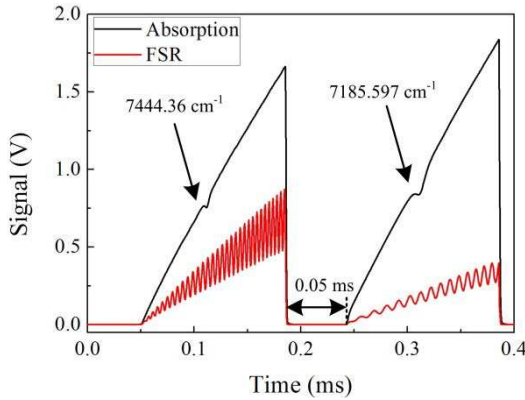
Fig. 10. Absorption and FSR signals obtained by the TDM scheme.
