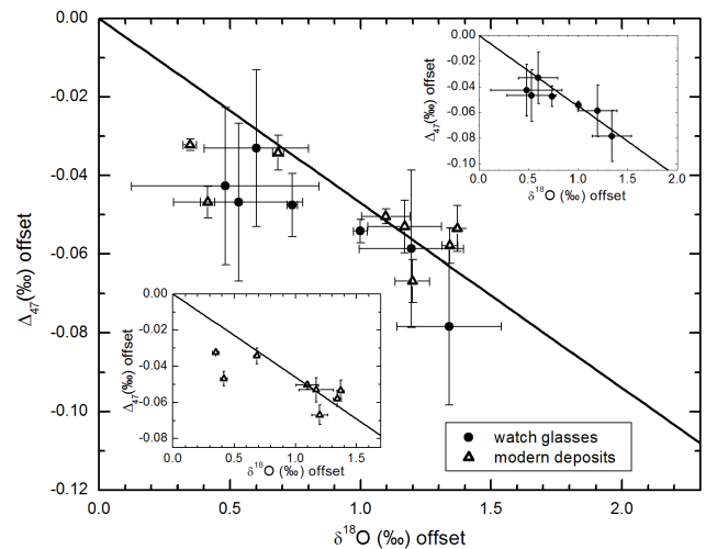
Fig. 1. \Delta_{47} offset versus \delta^{18}\text{O} offset in different sets of modern cave deposits. The thick line is a linear error-weighted fit through all modern calcites. It reflects the variable degree of kinetic isotope fractionation and assumes that \Delta_{47} and \delta^{18}\text{O} vary together in both \text{CO}_2 degassing and hydration/hydroxylation reaction. The insets depict separate fits of calcite precipitates on watch glasses from Bunker Cave (upper inset) and modern calcites from adjacent caves (lower inset) resulting in similar slopes (watch glasses: -0.055 \pm 0.002 , modern deposits excluding watch glasses: -0.046 \pm 0.007 , all modern calcite precipitates: -0.047 \pm 0.005 ). The origin is defined as the expected equilibrium for both \delta^{18}\text{O} and \Delta_{47} .
