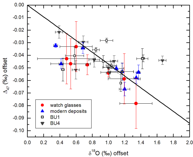
Fig. 2. \Delta_{47} versus \delta^{18}\text{O} offsets for Holocene stalagmites BU1 and BU4 as well as modern speleothems (adapted from Kluge and Affek, 2012). The offsets of the Holocene BU1 and BU4 samples were calculated for illustration purposes assuming a constant drip-water \delta^{18}\text{O} value of -7.9\text{‰} and a constant temperature of 9.5\text{°C} ( 8.5\text{°C} for BU4-9). The straight line is the slope obtained from a linear fit of modern calcite precipitates (Fig. 1). Deviations of BU1 and BU4 samples from this line are likely due to slight deviations of the actual climatic parameters from the assumption of a constant temperature and drip-water \delta^{18}\text{O} value (see Supplement Sect. A3).
