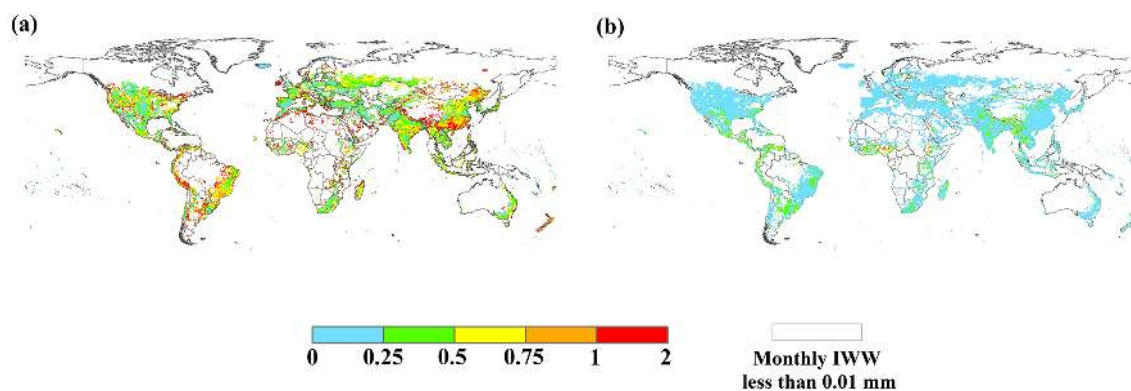
Figure 8. Coefficient of variation (CV) in multi-annual average irrigation water withdrawal caused by (a) multi-model framework and by (b) multi-forcing data, and areas with monthly mean irrigation water withdrawal (IWW) less than 0.01 mm are not taken into consideration.
