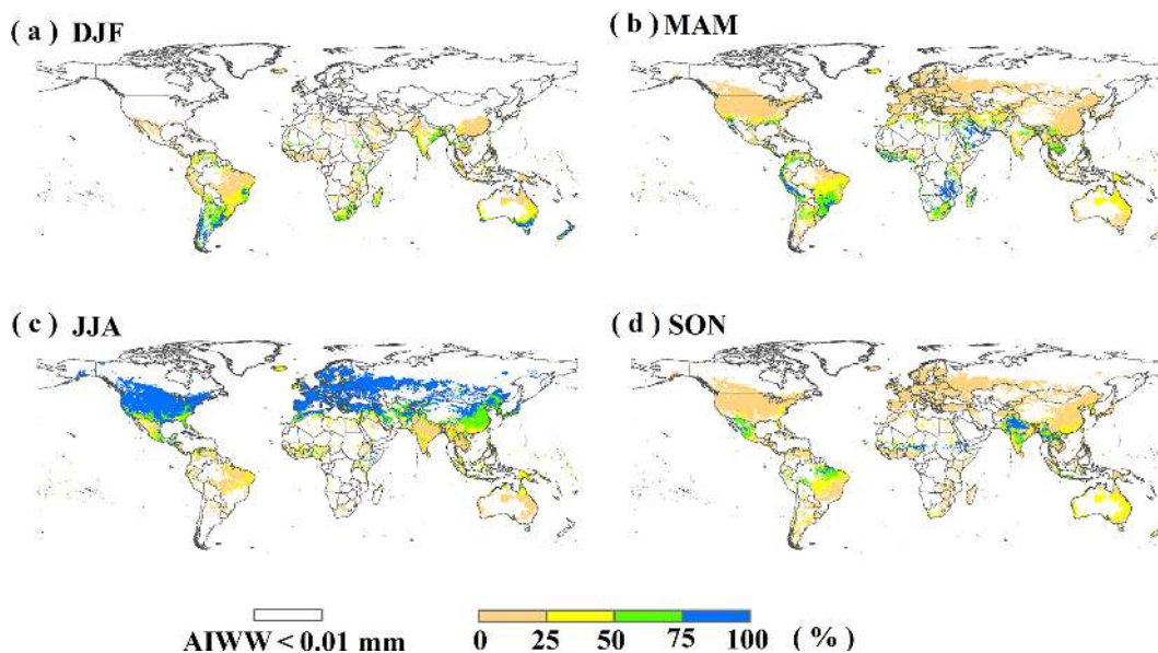
Figure 4. Relative seasonal distribution of global irrigation water withdrawal over the period 1971–2010 based on the ensemble mean of four GHMs: December to February (DJF), March to May (MAM), June to August (JJA), and September to November (SON), and grids with annual irrigation water withdrawal (AIWW) less than 0.01 mm are not taken into consideration.
