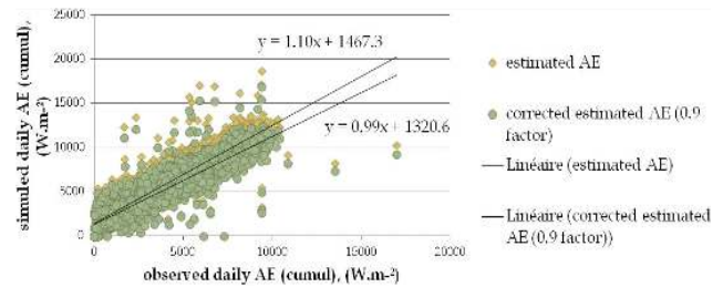
Fig. 4. Comparison of estimated AE (from Eq. 3) and corrected AE (from Eq. 6). All data and all sites are considered.
