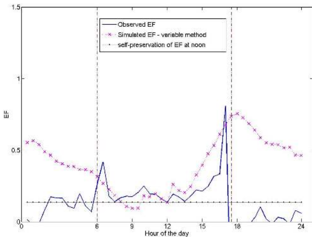
Fig. 7. Observed and simulated (Eq. 7) EF diurnal fluctuations: example for day of year 73 for the Morocco 2004 dataset.
