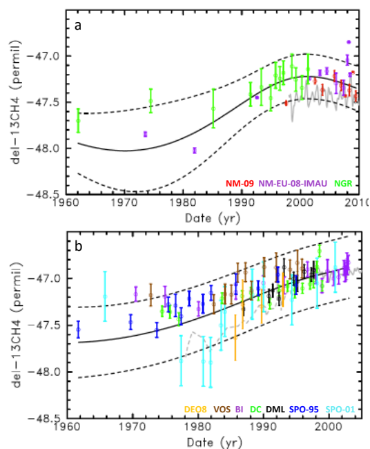
Fig. 6. Firm air \delta^{13}\text{C}(\text{CH}_4) datasets corrected for isotopic fractionation in firn (diffusion and gravitational settling) as a function of age. (A) NH sites, NM-EU-08 (purple), NM-09 (red), NGR (green). (B) SH sites, DE08 (orange), BI (purple), SPO-95 (dark blue), SPO-01 (light blue), DML (black), DC (green), VOS (brown). The dashed grey line in (B) represents air-archive data from Cape Grim (Francey et al., 1998) and the solid grey lines represent continuous atmospheric monitoring data from the NOAA-ESRL network. Note that the age spread of each data point is not presented here in order to keep the figure readable.
