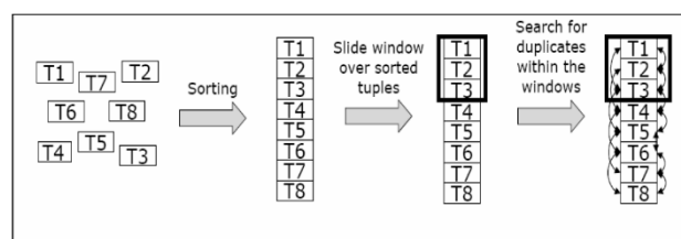
Fig. 2 Windowing [6]
