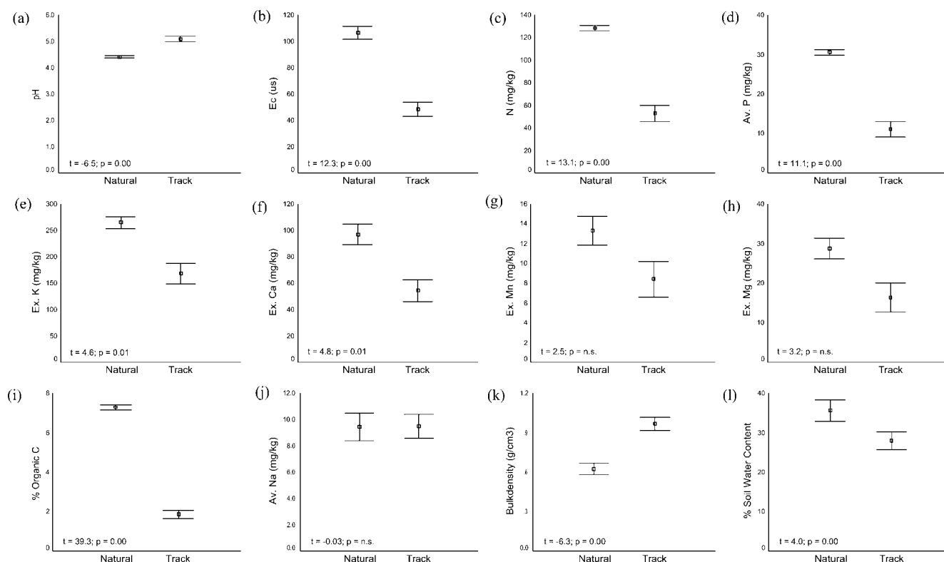
FIGURE 6. Soil nutrients and physical characteristics for ten 1 m 2 paired quadrats sampled along a closed track and in adjacent natural vegetation in the Kosciuszko alpine area: (a) pH, (b) conductivity, (c) nitrogen, (d) phosphorus, (e) potassium, (f) calcium, (g) manganese, (h) magnesium, (i) organic carbon, (j) sodium, (k) bulk density, and (l) soil water content. Significance values are Bonferroni adjusted paired t -test results.
