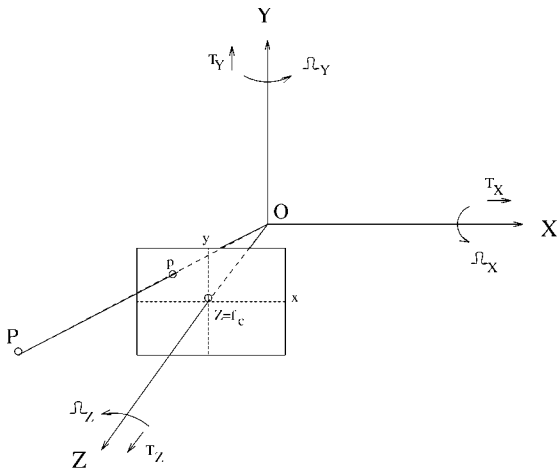
Fig. 1. The coordinate system. The coordinate system (X, Y, Z) is attached to the camera, and the corresponding image coordinates (x, y) on the image plane are located at Z = f_c . A point P = (X, Y, Z)^t in the world is projected onto an image point p = (x, y)^t . T = (T_X, T_Y, T_Z)^t and \Omega = (\Omega_X, \Omega_Y, \Omega_Z)^t represent the relative translation and rotation of the camera in the scene.
