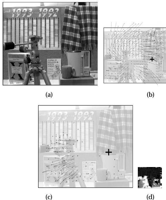
Fig. 2. The optical flow before and after 2D alignment of the image region corresponding to the wall. The camera was translating and rotating, and the real FOE is marked by \{+\} . The optical flow is given only for display purposes, and it is not used for the registration. (a) One of the frames in the sequence. (b) The optical flow to another frame (before registration), overlaid on Fig. 2a. The FOE mistakenly appears to be in the wrong location (in the middle of the frame). This is due to the ambiguity caused by the camera rotation around the Y-axis. (c) The optical flow after 2D alignment of the wall. The flow is induced by pure camera translation (after the camera rotation was canceled), and points to the correct FOE. (d) An example of depth map, computed using the recovered ego-motion. Bright regions correspond to near objects.
