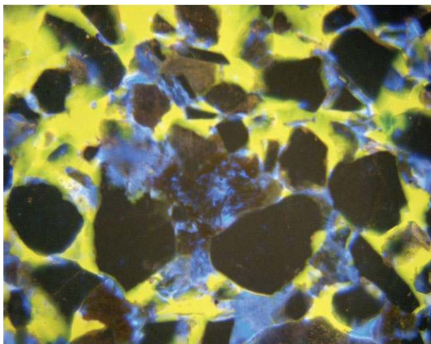
Figure 1. A thin section through an oil-bearing sandstone showing how the oil (dyed blue) and water (dyed yellow) occupy the spaces between the sand grains. The pore space was originally filled with water before oil migrated into the reservoir rock displacing the water.
