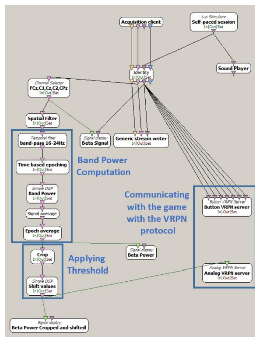
Figure 9: OpenViBE scenario to run the actual use-the-force game, after it is calibrated. This scenario computes the beta band power of the user in the Laplacian Cz channel, threshold it to detect a possible beta rebound following executed or imagined foot movement, and transmit the resulting command to an external 3D application (rendering and animating the spaceship) using the VRPN protocol.
