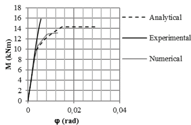
Fig. 21. M-\phi relationship of specimen M12C15025I8
