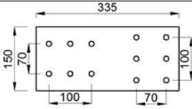
Fig. 8. Gusset plate of specimen M12C15025I10
