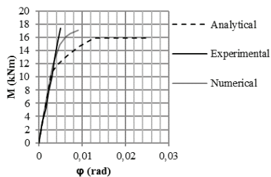
Fig. 20. M-\phi relationship of specimen M12C15025I10
