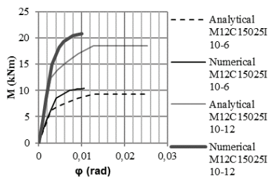
Fig. 22. M-\phi relationship of specimens M12C15025I10-6 and M12C15025I10-12
