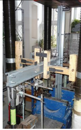
Fig. 7. Test specimen
