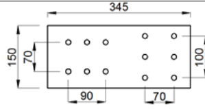
Fig. 9. Gusset plate of specimen M12C15025I8
