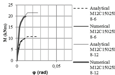
Fig. 23. M-\phi relationship of specimens M12C15025I8-6 and M12C15025I8-12
