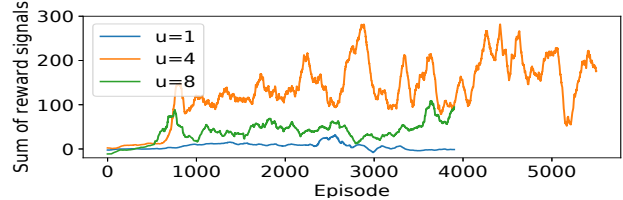
(b) Learning curves of agents with various update length and fixed l as 8. The agents are trained on the terrain without obstacles otherwise the agents with u=1 or 8 do not learn to walk.
