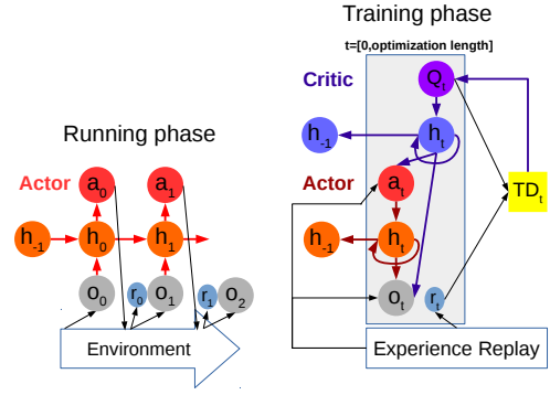
Fig. 2: Recurrent deterministic policy gradient (RDPG).
