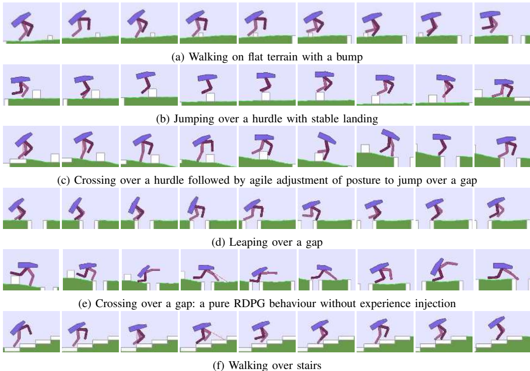
Fig. 10: Terrain specific agile behaviors generated by our RDPG agent trained with experience injection.
