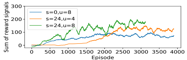
(a) Learning curves of agents with various scanning interval lengths ( s ). Optimization length is set as 8.
