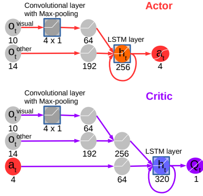
Fig. 6: Network design of Actor and Critic.
