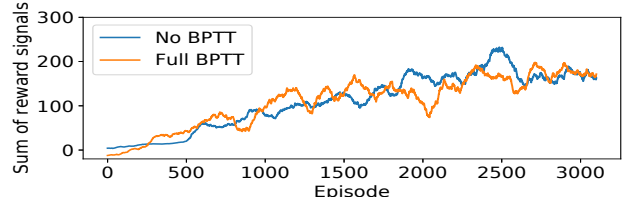
(b) Effect of BPTT truncation on learning performance. Same hyperparameters are set as u = l = 8, s = 24 .
