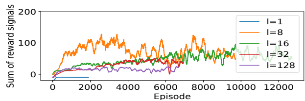
(a) Learning curves of agents with various optimization length ( l ). Update length ( u ) is set as half of the optimization length.
