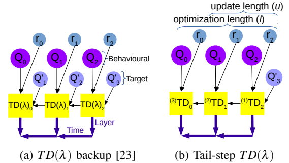
Fig. 4: TD measurement in a subtrajectory. Thick purple line: backpropagation of Critic update gradient.
