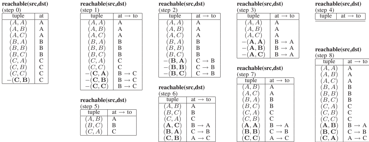
Fig. 5. DRed algorithm: over-delete and re-derive steps after deletion of link(C,B) .
