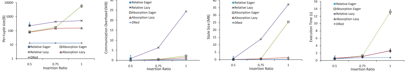
Fig. 7. reachable query computation as insertions are performed
