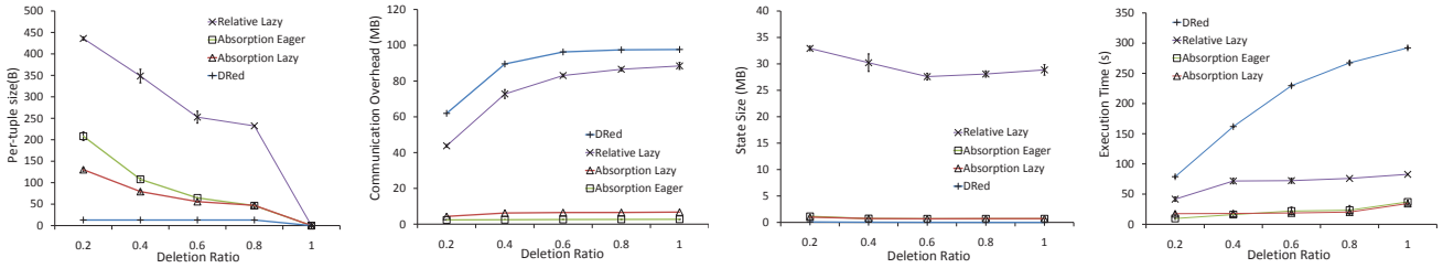
Fig. 8. reachable query computation as deletions are performed
