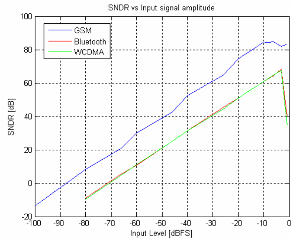
Figure 7. SNDR versus input signal amplitude
