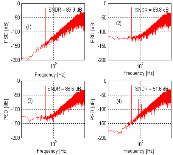
Figure 5. PSD of (1) the ideal modulator; (2) with sampling jitter, \Delta\tau = 4 ns; (3) with kT/C noise, C_s = 1.25 pF; (4) with SR = 50 V/ \mu s.
