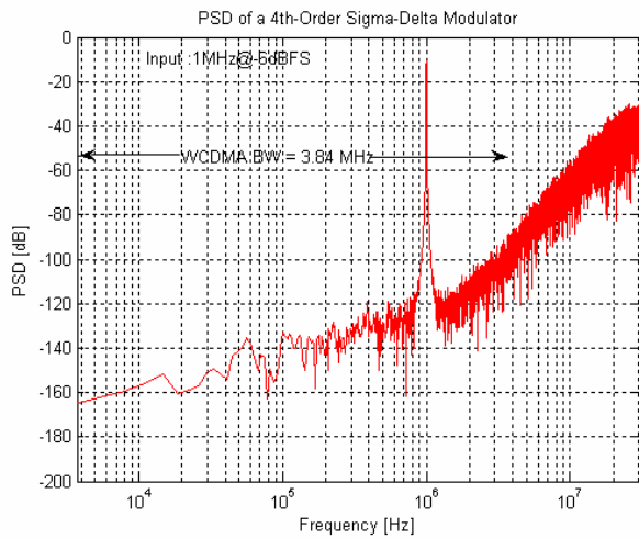
(b) Modulator output spectrum in WCDMA mode
