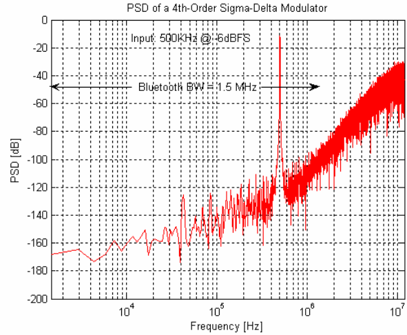
(c) Modulator output spectrum in Bluetooth mode
