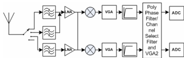
Figure 1. Reconfigurable low IF-zero IF receiver architecture for GSM/WCDMA/Bluetooth standards
