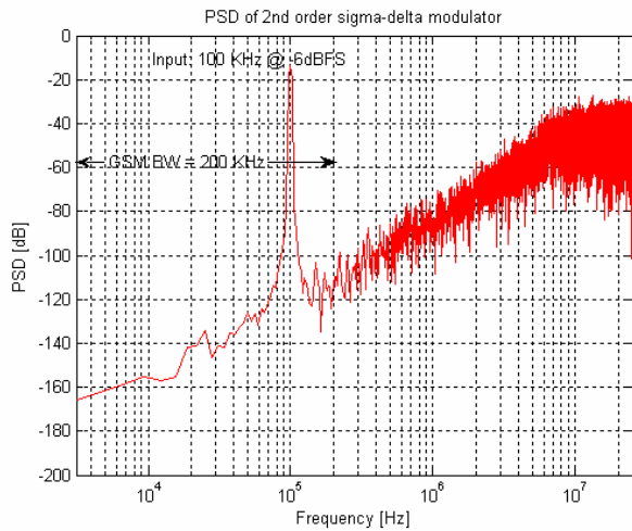
(a) Modulator output spectrum in GSM mode
