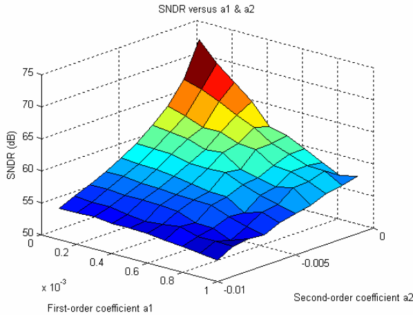
Figure 4. 3D Simulation for non-linear dc gain
