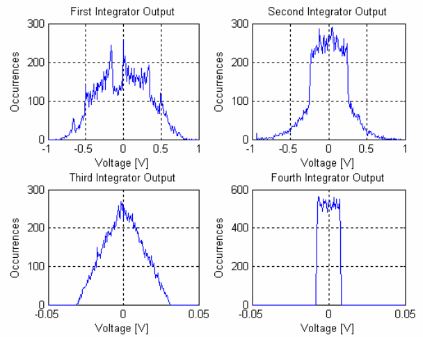
Figure 3. Integrator output swings
