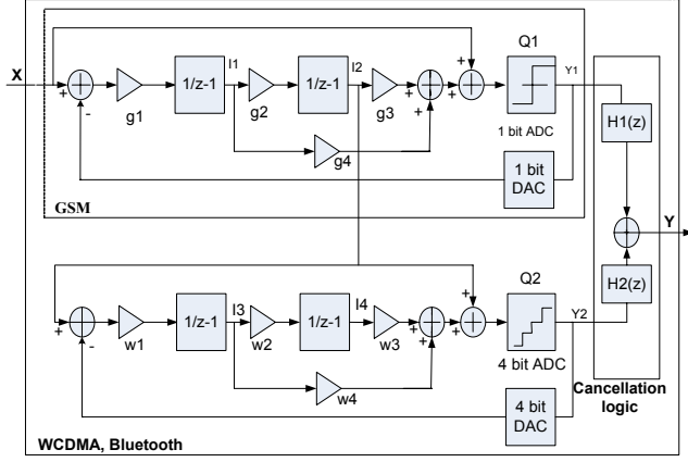
Figure 2. Block diagram of a triple-mode sigma-delta modulator
