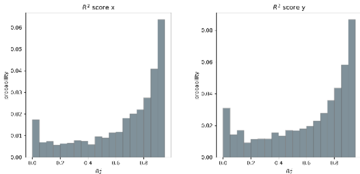
Fig. 4. Coefficient of determination R^2 for x and y for all training tracklets of the World H-H TrajNet challenge.
