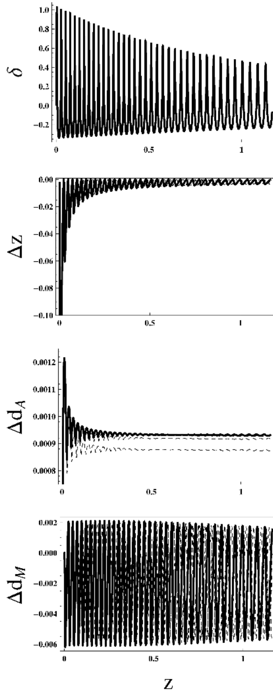
Figure 7. The effect of inhomogeneities with \delta \approx 1 today, periodic on a scale of 100 Mpc.
