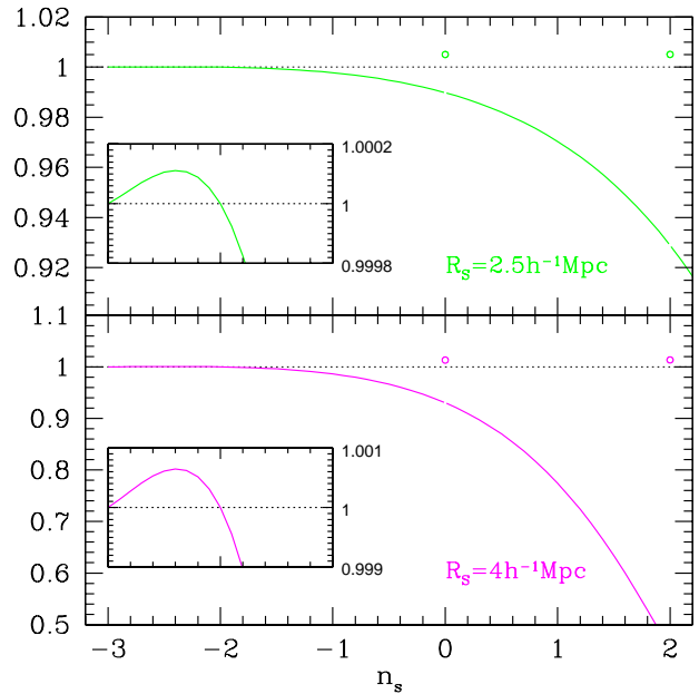
FIG. 7: Cross-correlation coefficient r_\xi(r) for powerlaw power spectra P_\delta(k) \propto k^{n_s} as a function of the spectral index n_s . Results are shown at a single separation r = 100 h^{-1} \text{Mpc} , for density peaks identified at the smoothing scale R_S = 2.5 (top) and 4 h^{-1} \text{Mpc} (bottom). The insert is an enlarged view of r_\xi in the range -3 < n_s < -1 . Notice the discontinuities at n_s = 0 and 2 , at which the cross-correlation coefficient is slightly larger than unity.
