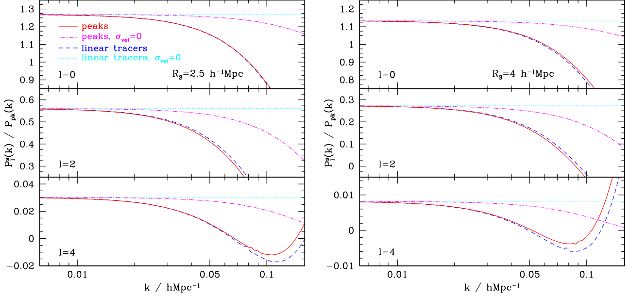
FIG. 4: Fourier space multipoles \mathcal{P}_\ell^s in unit of P_{\text{pk}}(k) as a function of wavenumber for the density peaks and for the linearly biased tracers with same value of b_\nu^{\text{Eul}} . The dotted-dashed (peaks) and dotted curves (linear tracers) are the results without including the velocity damping kernel (assumed to be a Gaussian, see Sec. III C), while the solid (peaks) and dashed (linear tracers) curves represent the multipoles when the Gaussian dispersion is included. For density peaks, \mathcal{P}_\ell^s(k) exhibit a strong k -dependence even upon removal of the damping term.
