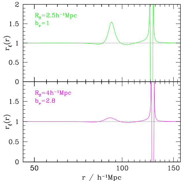
FIG. 6: The cross-correlation coefficient r_\xi(r) for density peaks identified at the smoothing scale R_S = 2.5 and 4 h^{-1}\text{Mpc} (upper and lower panel, respectively). There is significant stochasticity only at the zero-crossings of the auto and cross-correlation functions and across the BAO, where the derivatives of the density correlation \xi_0^{(1)} and \xi_0^{(2)} are not negligible [29].
