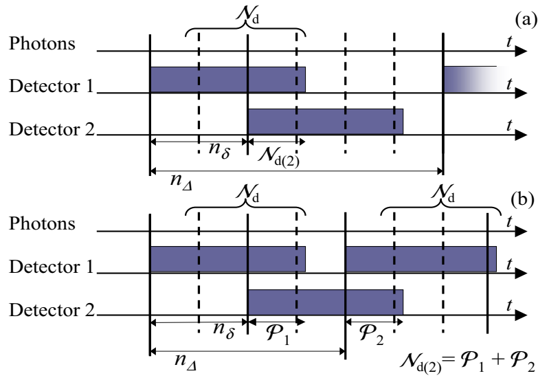
Figure 4. The effective deadtime of D1. Case (a) the time interval between two subsequent counts of D1, n_\Delta \geq n_\delta + \mathcal{N}_d , with n_\delta the time interval between the count of D1 and the subsequent photon counted by D2 during the deadtime of D1, and T_d the actual single detector deadtime. Case (b) n_\Delta < n_\delta + \mathcal{N}_d . In this second, case two terms, \mathcal{P}_1 and \mathcal{P}_2 contribute to the final deadtime.
