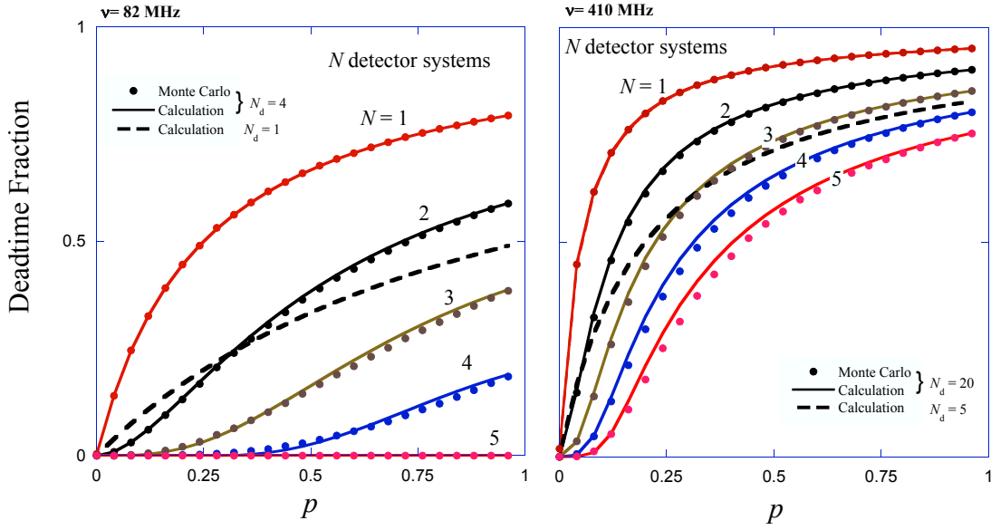
Figure 5. Deadtime Fraction versus probability of detection per pulse for pools of up to 5 detectors, for detectors each with T_d = 50 ns, with a pulsed source with repetition rate of (a) 82 MHz ( \mathcal{N}_d = 4 ), and (b) 410 MHz ( \mathcal{N}_d = 20 ). Dots represent the Monte Carlo simulations, while solid lines are the calculated values according to the here presented theory. For comparison, a single-detector-DTF (broken line) with a reduced deadtime of 12.5 ns, corresponding to (a) \mathcal{N}_d = 1 and (b) \mathcal{N}_d = 5 are shown.
