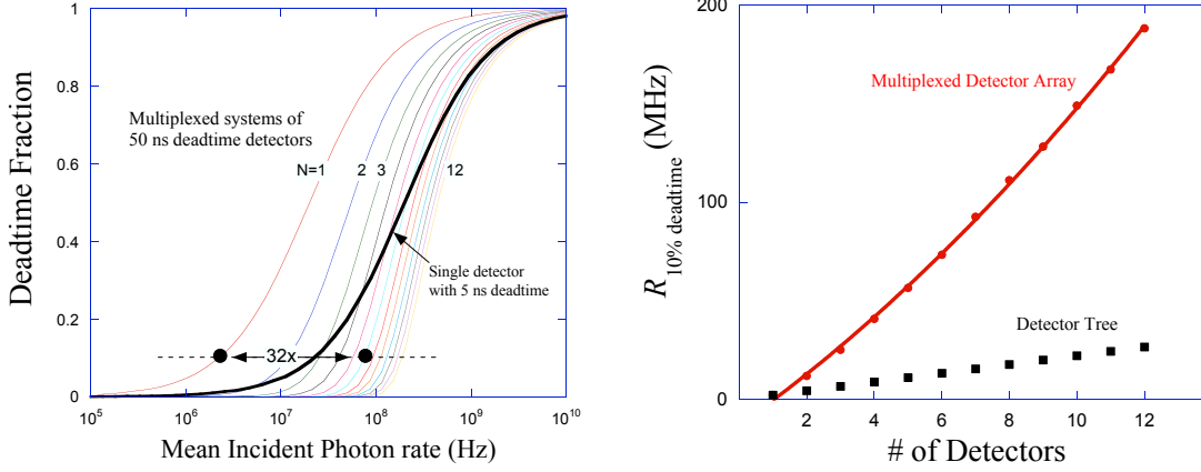
Figure 3. a.) DTF versus mean incident photon rate shown for systems of 1 to 12 detectors, all with 50 ns deadtimes. The dashed horizontal line shows the 10 % DTF level that is often the practical limit for detector operation. The DTF for a single detector with 5 ns deadtime is shown for comparison (thick line). As an example of the advantage of the scheme, the two points illustrating that with 6 detectors the system would be able to operate at a 32 times larger incident photon rate than a single detector, while maintaining that 10 % DTF. b.) R_{DTF=10\%} (dots) versus number of detectors in the detector pool, along with a fit to a 2nd order polynomial (line). For comparison the dependence of R_{DTF=10\%} for a detector tree is also shown (squares).
