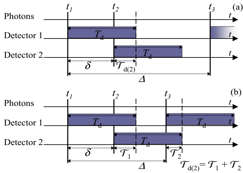
Figure 2. The effective deadtime of D_1 . Case (a) the time interval between two subsequent counts of D_1 , \Delta > \delta + T_d , with \delta the time interval between the count of D_1 and the subsequent photon counted by D_2 during the deadtime of D_1 , and T_d the single detector deadtime. Case (b) \Delta < \delta + T_d . In this second case two terms, \mathcal{T}_1 and \mathcal{T}_2 contribute to the final deadtime. Dark shaded regions represent the deadtime of the individual detectors.
