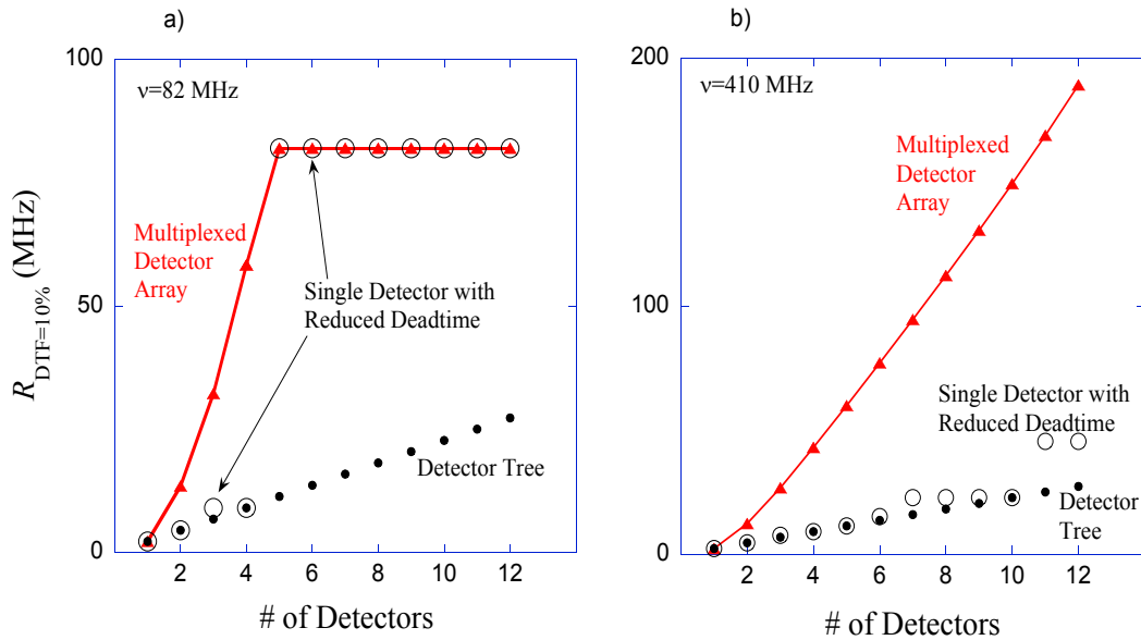
Figure 6. R_{DTF=10\%} (the incident rate at which the DTF reaches 10 %) of a multiplexed detector array (triangles), a single detector with reduced deadtime (open circles), and a detector tree configuration (dots) for pulsed sources with repetition rates of (a) 82 MHz, (b) 410 MHz. The single detector points in (a) and (b) are plotted versus 1/N reduction in T_d .
