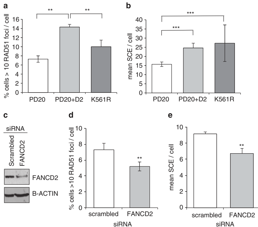
Figure 5. Endogenous RAD51 foci and SCE levels are decreased in FANCD2-deficient PD20 and FANCD2-depleted MRC5VA cells. (a) Quantification of RAD51 and (b) SCE formation in the FA-derived cell line PD20 and wild-type FANCD2 (PD20-D2) and FANCD2 monoubiquitination mutant (PD20-K561R) complemented PD20 cells. (c) Western blot for FANCD2 in MRC5VA cells treated for 48 h with scrambled or FANCD2 siRNA. (d) Quantification of RAD51 foci and (e) SCE formation in FANCD2-depleted MRC5VA cells. Average and s.d. of three repeats is shown. Significance was calculated using Student's t -test; ** P < 0.01 and *** P < 0.001 . SCE is expressed as the number of SCE observed/diploid genome. Where polyploidy existed, numbers were adjusted accordingly.
