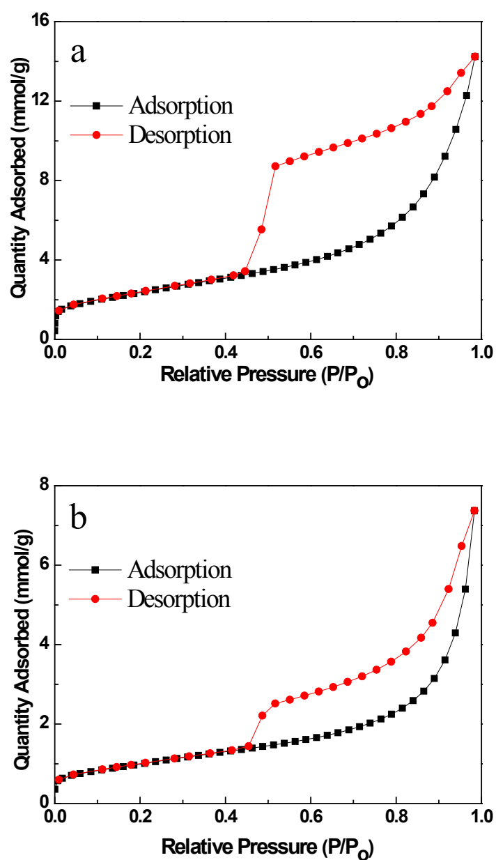
Fig. S2 Nitrogen adsorption and desorption isotherms of (a) RGO/Ni-1 and (b) RGO/Ni-2 nanocomposites.
