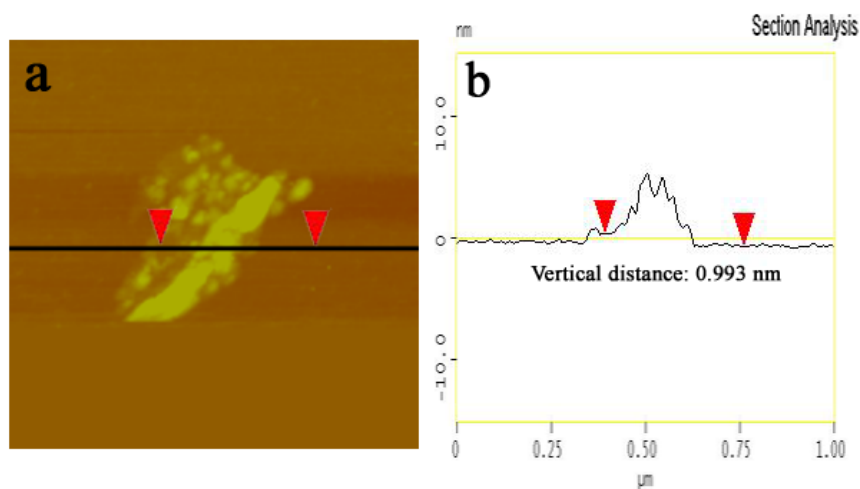
Fig. S1 (a) AFM image of RGO/Ni-1 nanocomposites and (b) the cross section analysis.
