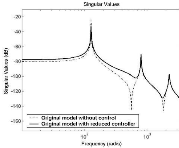
Figure 6: Comparison of singular value diagrams: original model without control and controlled by the reduced controller.
