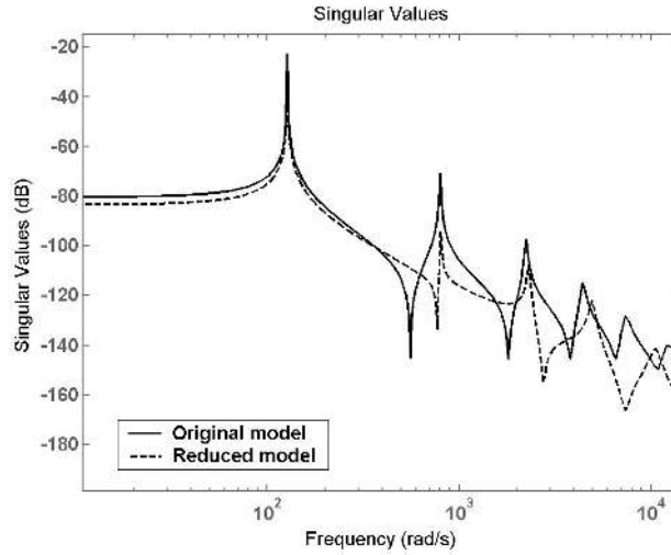
Figure 5: Comparison of singular value diagrams: original model and reduced model.
