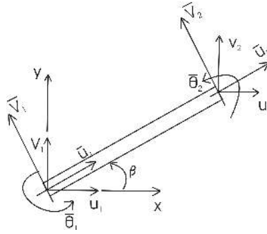
Figure 2: Element in global coordinates system.
