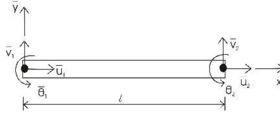
Figure 1: Bi-dimensional finite element.
