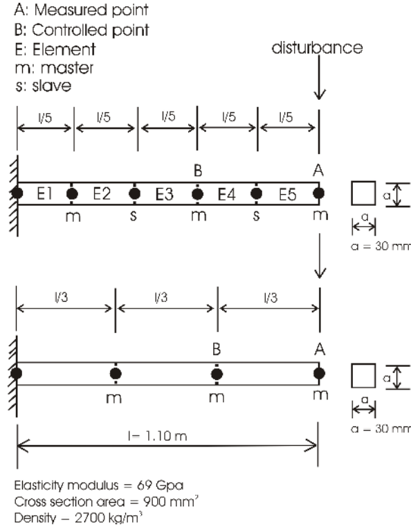
Figure 4: Original structure with 15 degrees of freedom that was reduced to 9 master degrees of freedom.
