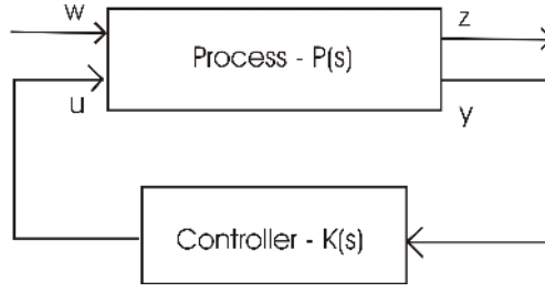
Figure 3: Process and H_\infty controller schemes.
