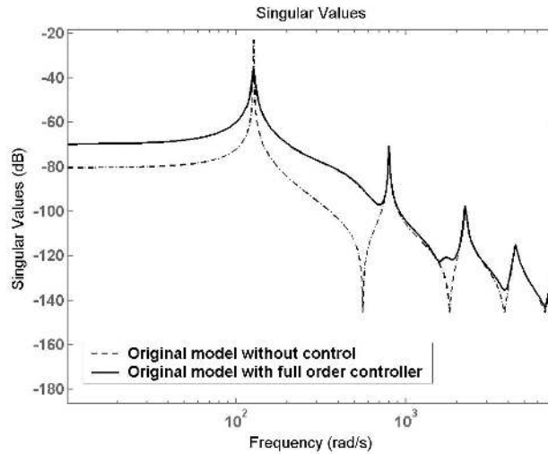
Figure 7: Comparison of singular value diagrams: original model without control and controlled by a full order controller.
