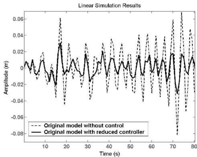
Figure 8: Comparison of time responses for the displacement at non fixed end: original model without control and controlled by the reduced order controller.
