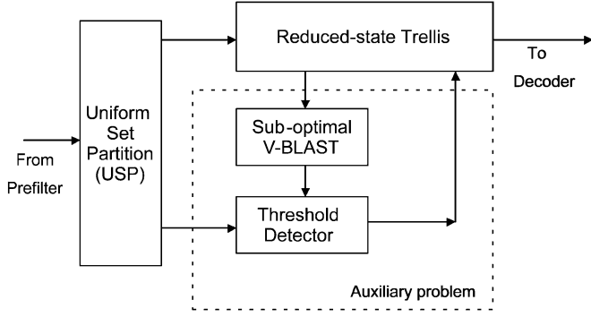
Fig. 3. Block diagram of JRSSD structure.
