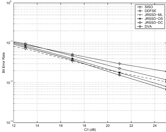
Fig. 9. BER comparison for an interference-limited RA100 channel, DIR = 15 dB.
