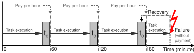
Figure 5. Hour-boundary checkpointing
