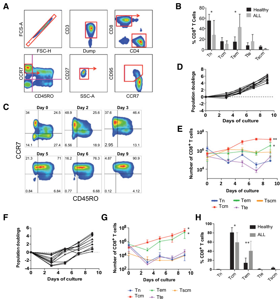
Figure 1. T cells progressively differentiate over time during ex vivo culture. A , Gating strategy used to identify Tn, Tscm, Tcm, Tem, and Tte subsets. The arrow identifies which subset was examined further. B , The proportion of CD8 + T-cell subsets freshly isolated from the peripheral blood of healthy donors ( n = 9 ) and individuals with ALL ( n = 9 ) calculated using the gating strategy shown in A . *, P < 0.05 . C , Representative plots of CART19 cells at the specified timepoints during culture. Pregated for live CD3 + CD8 + T cells as shown in A . D , Ex vivo proliferation of healthy donor T cells following stimulation with anti-CD3/CD28 microbeads. Total viable T cells were enumerated by flow cytometry using bead-based counting. Each donor is represented by a separate line. Dotted line: 0 population doublings. E , Absolute counts of CD8 + T cells subsets over time in cultures of healthy donors shown in D . Data are plotted as mean \pm SD. **, P < 0.01 ; *, P < 0.05 comparing d3 vs. d9. F , Ex vivo proliferation of T cells from ALL patients stimulated and enumerated as in D . G , Absolute counts of CD8 + T cells from ALL patients as shown in F . *, P < 0.05 ; **, P < 0.05 comparing d3 vs. d9. H , The proportion of CD8 + T cells in healthy donors and ALL patients analyzed on day 9 of culture. *, P < 0.05 ; **, P < 0.01 . All comparisons were analyzed by Wilcoxon matched-pairs signed rank test.
