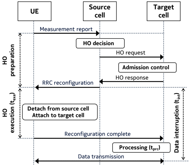
Fig. 1. Break-before-make intra-LTE handover procedure. Based on [13].
