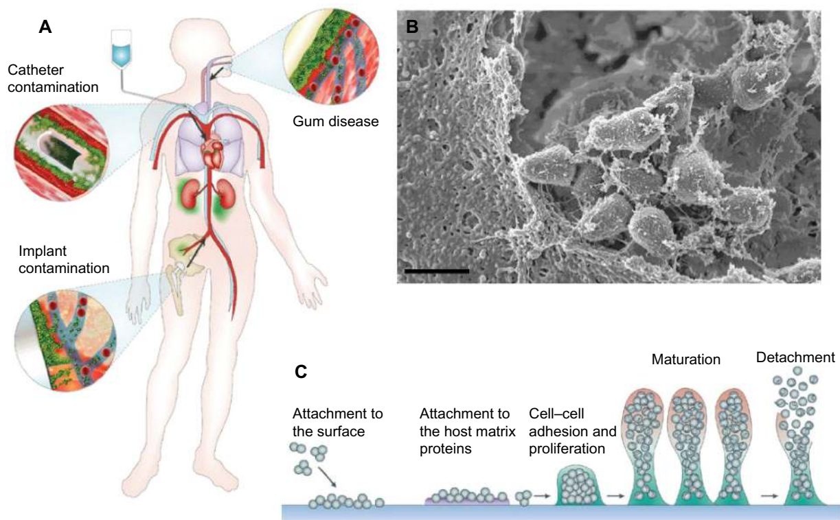
Figure 1 Biofilm pathogenicity in humans is mediated by dissemination and biofilm matrix formation. (A) Possible routes of biofilm dissemination around the body originating from sites such as gum disease, catheter, or implant contamination. 12 (B) Scanning electron micrographs (SEM) of biofilm matrix, offering protection of resident bacteria from eradication, imaged from a clinical endotracheal tube identified as Streptococcus pneumoniae . Scale bar shown is 1 \mu m. (C) Schematic of biofilm-mediated device-related infection, starting with bacterial attachment to a device or adsorbed host proteins, leading to biopolymer mediated cell-cell adhesion, maturation, and eventual detachment leading to the spread of infection. 66
