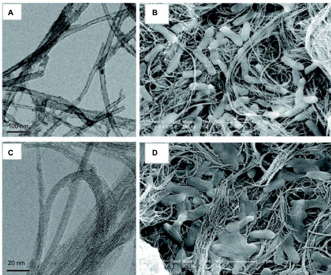
Figure 5 The diameter of the carbon nanotubes determined by transmission electron microscopy (A and C) predicts antimicrobial behavior as visible in scanning electron micrographs (B and D). 53 A mat-like surface made of multiwalled carbon nanotubes (A) inactivates a small percentage of Escherichia coli , visible as abnormal and flattened bacteria on the surface (B). Single-walled carbon nanotubes (C), having a smaller diameter, inactivate a greater percentage of bacteria, causing significant structural disruption and bacterial death (D).
