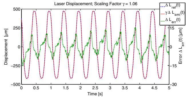
Fig. 10 The laser displacement measured via SMI and scaled by \gamma = 1.06 (heavy solid curve), the reference LDV measurement (heavy dashed curve), and their difference \Delta L_{\text{err}}(t) = \gamma \Delta L_{\text{smi}}(t) - \Delta L_{\text{ref}}(t) (thin curve). The difference has been shown explicitly, because the SMI and LDV displacement measurements are almost identical.
