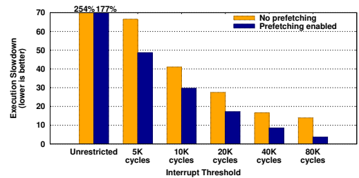
Figure 6. Overhead sensitivity of monitoring art .
