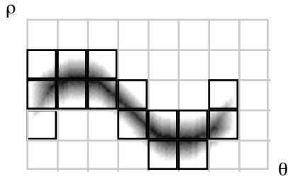
FIG 4 : Fuzzy sine curve set fitted to a fuzzy image box X_i \times Y_j .
