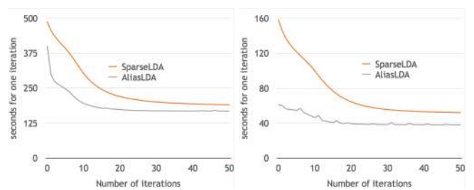
Figure 3: Runtimes of SparseLDA and AliasLDA on PubMedSmall (left) and NyTimes (right).
