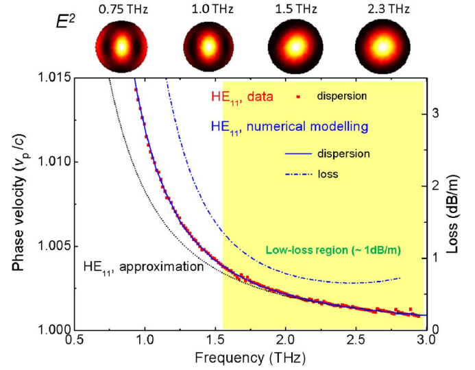
Fig. 6. Dispersion characteristics for the HE_{11} mode in the 1.8 mm diameter dielectric-lined hollow metallic waveguide. The PS coating is modelled as a 17 \mu\text{m} thick lossless dielectric layer. The experimental characteristics measured by THz-TDS are shown by red squares [18]. The dispersion curves are compared to the analytical approximation for the cutoff frequency of 0.128 THz. The losses in the metallic walls are estimated numerically. At low frequencies, the numerically modeled HE_{11} mode profiles show that significant energy density is distributed near metallic walls.
