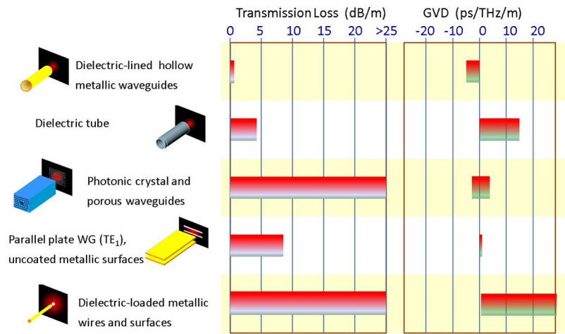
Fig. 1. Common THz waveguides and their estimated transmission loss and dispersion characteristics in the region of 1–2 THz [7]–[23].
