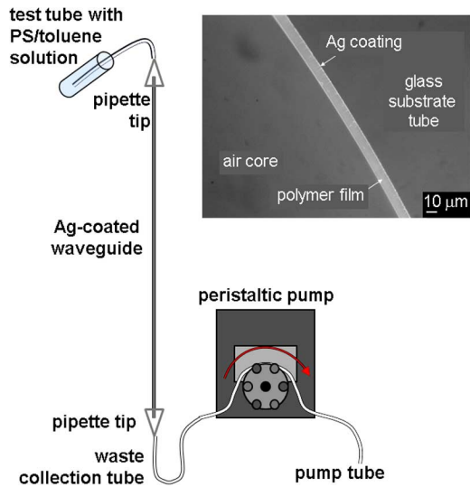
Fig. 2. A schematic diagram of the apparatus used to deposit polymer thin films over Ag films. Inset: an optical micrograph of a 2.2 mm bore diameter Ag/PS waveguide showing the PS layer [38].
