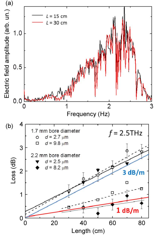
Fig. 5. (a) THz TDS spectra measured at the output of a 15 and 30 cm long Ag/PS waveguides (1.8 mm diameter) showing periodic features due to the mode interference. Narrow absorption lines are caused by water vapour ( \sim 50\% RH) inside the waveguide core. (b) Single frequency cutback loss measurements at 2.54 THz (far-infrared laser) [19]. The red and blue lines mark the transmission loss levels of 1 dB/m and 3 dB/m respectively.
