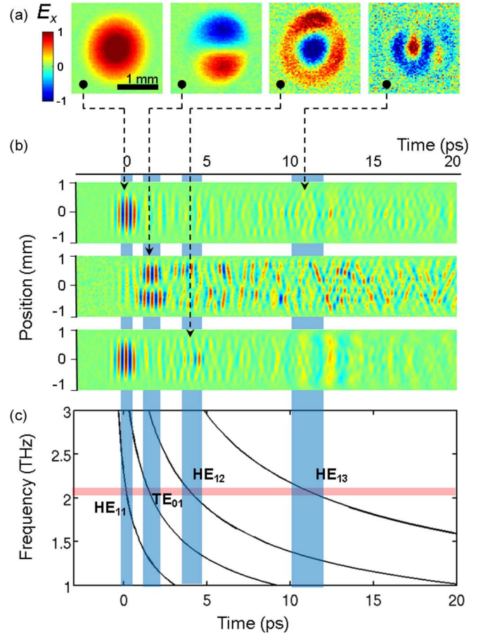
Fig. 4. Time-resolved near-field mode mapping. (a) Two-dimensional distributions of the electric field component E_x(x, y) are shown in the top row for various time delays corresponding to the arrival of different modes [18]. (b) Space-time maps at the output of the 133.5 mm long Ag/PS waveguide for three different coupling configurations: through a 1 mm diameter pinhole centered on the waveguide axis (top map); through the pinhole positioned off-axis as in Fig. 3 (middle map); and the uniform waveguide input illumination (bottom map). (c) Estimated temporal delay for higher order modes. The origin of the time axis t = 0 is chosen to mark the arrival of the dominant HE_{11} mode.
