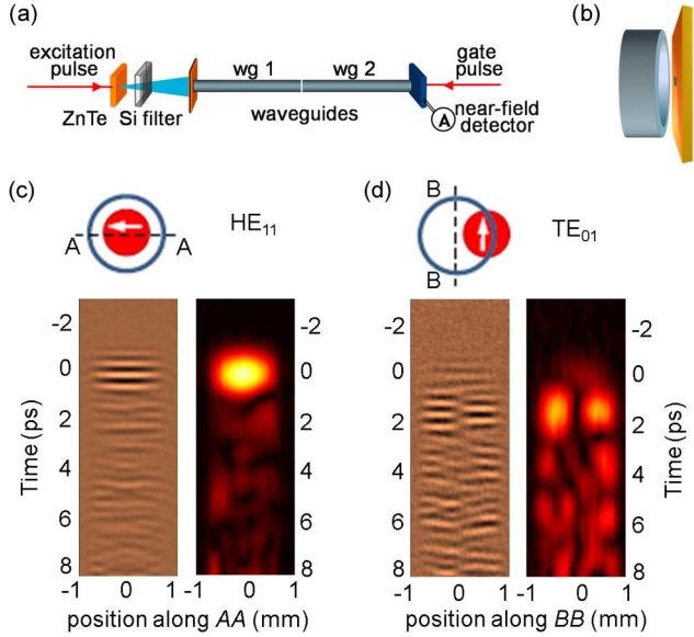
Fig. 3. (a) A schematic diagram of the experimental system for near-field mapping of waveguide modes. (b) A close-up of the waveguide output and the near-field field probe. (c) Space-time maps of the horizontal component of the electric field ( E_x ) for the HE_{11} mode at the output end of a 1.8 mm diameter 133.5 mm long Ag/PS waveguide: the left panel shows the measured electric field and the right panel shows the amplitude of the 2.3 THz component, near the pulse spectrum maximum. The HE_{11} mode is excited selectively by placing a 1 mm diameter pinhole at the waveguide entrance as shown in the schematic diagram. (d) Space-time maps and the excitation arrangement for the TE_{01} mode in the same waveguide.
