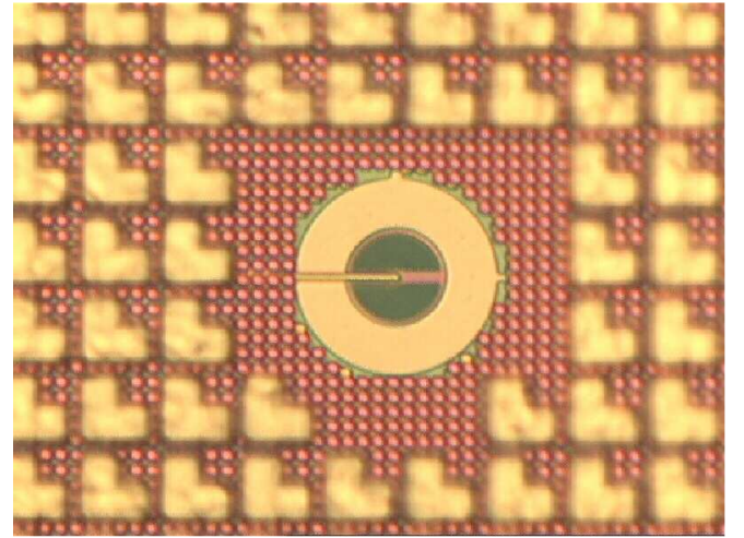
Fig. 5 SPAD Micrograph showing dummy fill elements
