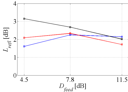
Figure 3. Reflection loss with the maximum offset; Conventional elliptical lenses with \epsilon_r = 2.5 (blue), \epsilon_r = 4 (red), and \epsilon_r = 12 (black).
