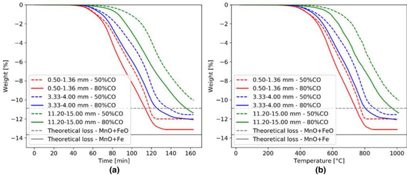
Fig. 14—Weight reduction behavior during non-isothermal (6 °C/min) reduction of Nchwanging ore as a function of a : time and b : sample temperature.
