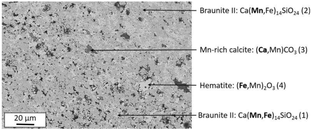
Fig. 13—Microstructure of Nchwanging ore (11.20 to 15.00 mm) obtained by backscatter imaging. Phases numbering correlate to chemical compositions shown in Table IX.
