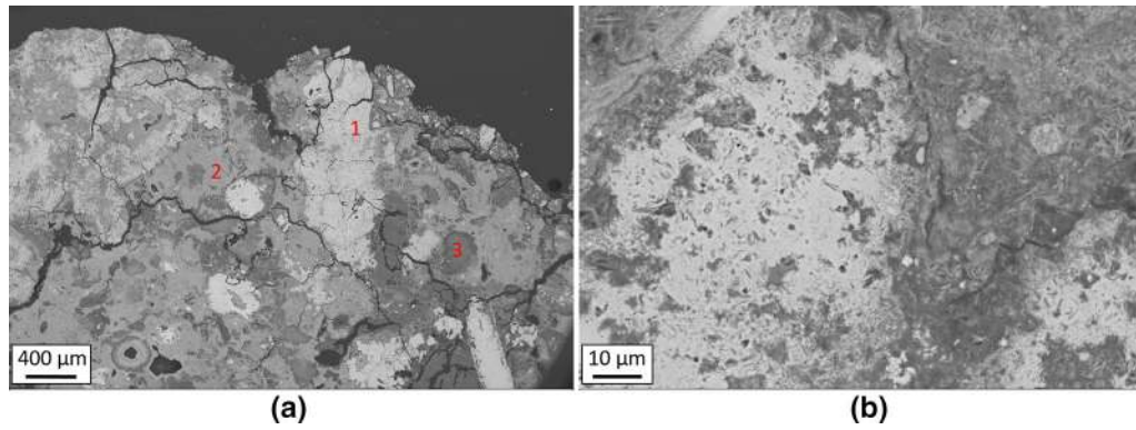
Fig. 8—Microstructure observed in Comilog ore particle (11.20 to 15.00 mm) reduced non-isothermally in 80 pctCO to 550°C. Reduction degree of 54 pct of higher manganese oxides to MnO according to chemical analysis. Overview including outer edge seen in A in scale of 400 \mu\text{m} , whereas B shows the center in scale 10 \mu\text{m} .
