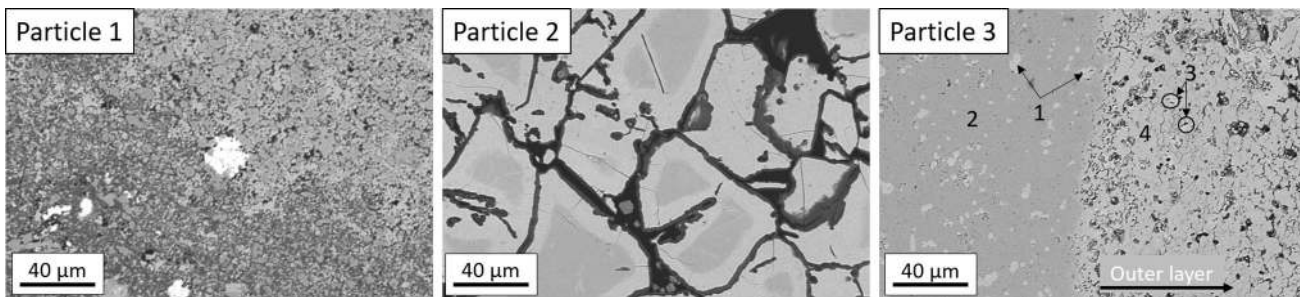
Fig. 18—Microstructure observed in three separate particles (11.20 to 15.00 mm) reduced non-isothermally in 80 pctCO to 800 °C. Reduction degree of 55 pct of higher manganese oxides to MnO according to chemical analysis.
