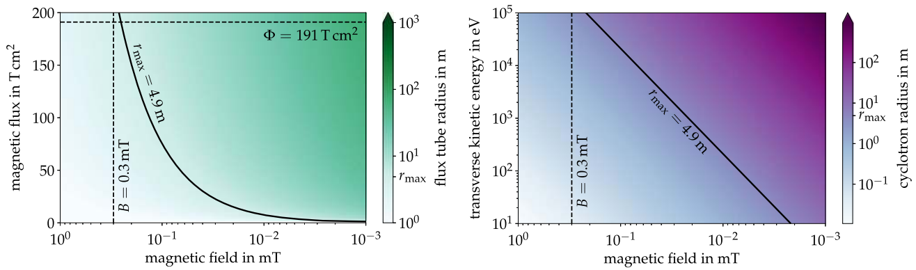
Fig. 3 Effects of the magnetic pulse on stored electrons. The magnetic field decreases towards the right in both plots; the dashed vertical lines mark the nominal field in the analyzing plane ( B_{\min} = 0.3 mT). Left: the flux tube widens when the magnetic field decreases according to Eq. (5). In this plot the magnetic flux corresponds to a flux tube cross-section with radius r_{\text{flux}} in the spectrometer center (indicated by color), and the solid line indicates the maximal vessel radius r_{\text{max}} = 4.9 m. Electrons stored in a flux tube region with r_{\text{flux}} > r_{\text{max}} are removed, and electrons
