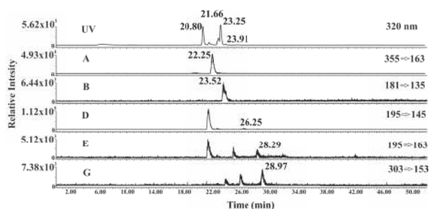
Figure 2 - Chromatogram of the lyophilized coconut water, by LC/MS/MS. Injection of 75 mg/mL solution of LCW in ACN 10% with formic acid 0.1%. The lyophilized CW was analyzed by Kinetex C18 XB (100 mm x 4.6 mm i.d., 2.6 \mu m of particle size, 100 \text{\AA} , Phenomenex, Torrance, CA), at 20°C, injection volume of 150 \mu L and flow rate of 0.175 mL/min. As for the mobile phase, it was used (a) formic acid 0.1% and (b) ACN with formic acid 0.1% following linear elution gradient: 0 min – 10% of (b), 25 min – 90% of (b), 30 min – 90% of (b), 43 min 10% of (b) – 50 min (stop), coupled with Quattro II mass spectrometer (Micromass, Manchester, UK) in positive mode ( \text{ESI}^+ ), 3.5 V on capillary, 25 V on cone, 15 psi of nebulizer gas, 350 L/h of dry gas, 300°C desolvation temperature and 100°C block source temperature. UV-320 nm; compounds detected - A: Chlorogenic acid; B: Caffeic acid; D: Ferulic acid; E: Methyl caffeate; G: Quercetin.
