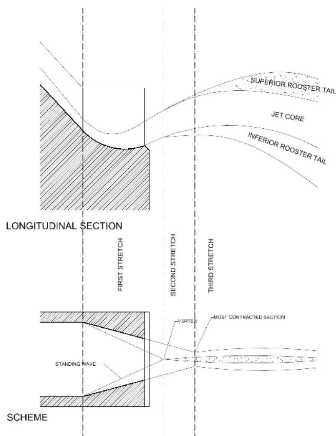
Figure 7. Aspect of effluent jet from Slit Buckets.
