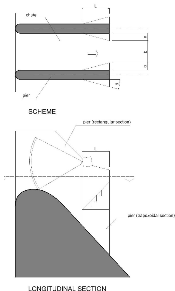
Figure 4. Scheme and typical sections of Flaring Pier.
