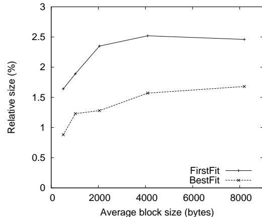
Figure 7: Effect of average block-size on relative size using REBL on the Slashdot data set.
