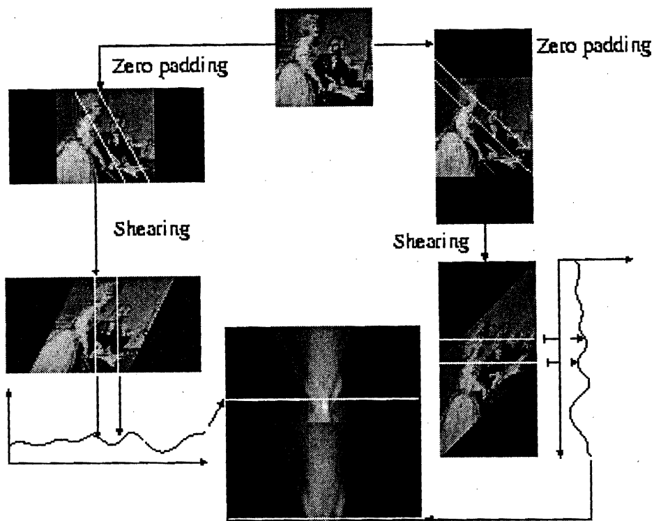
Fig. 18. Slant Stack Transform of an image.
