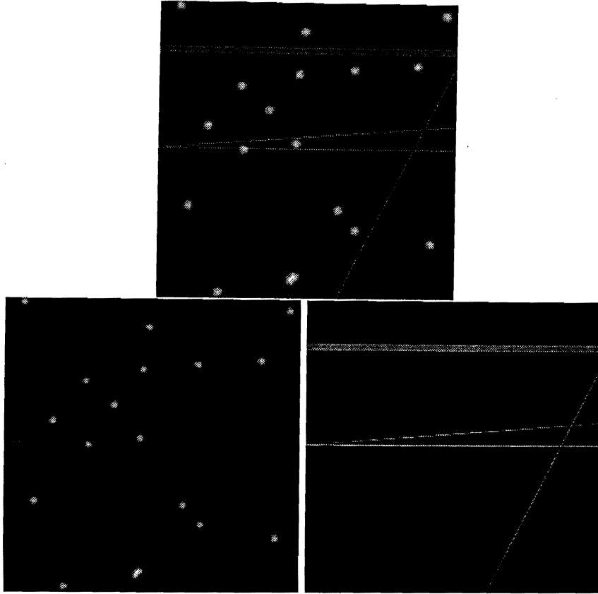
Fig. 25. Top, original image containing lines and Gaussians. Bottom left, reconstructed image for the à trous wavelet coefficient, bottom right, reconstructed image from the Ridgelet coefficients.
