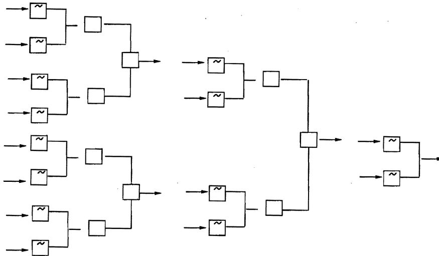
Fig. 2. 1D undecimated wavelet transform.
