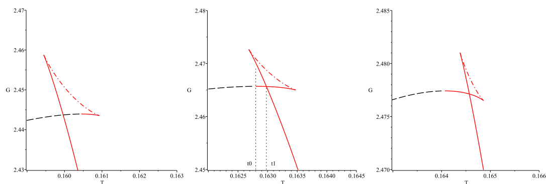
Figure 4. Reentrant phase transition: Gibbs free energy: k = 1 , e = q = 1 . These plots show the Gibbs free energy for P = 0.031, 0.0313 and 0.032 (left to right). Due to positivity of entropy constraints, one branch becomes unphysical below a certain temperature, which changes depending on the pressure—in the plots, this is shown with the dashed black curves. For a certain window of pressures we see the behaviour exemplified by the center figure. Such a configuration leads to a reentrant phase transition, since a monotonic variation of the temperature leads to a zeroth-order large/small black hole transition at t_0 , followed by a first order small/large black hole transition at t_1 .
