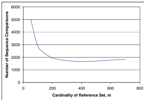
Figure 10: Impact of m : Number of comparisons of MP-D for DNA sequence database for values of m . The number of references is 8 and query range is 8.
