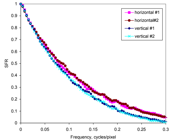
Figure 9. Improved results based on pooled slope estimates
