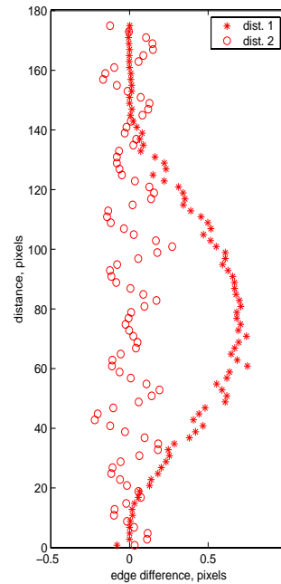
Figure 5. Edge displacement observed because of barrel lens (1) and(2) ripple type distortion
