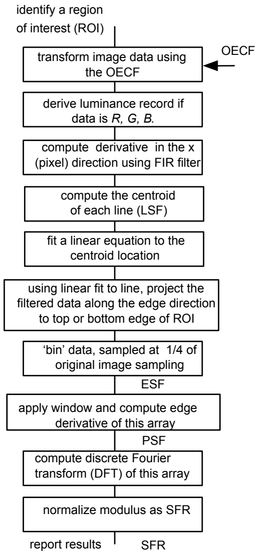
Figure 1. Description of the ISO 12233 spatial frequency response evaluation method. The edge is assumed to be oriented in a near-vertical direction.
