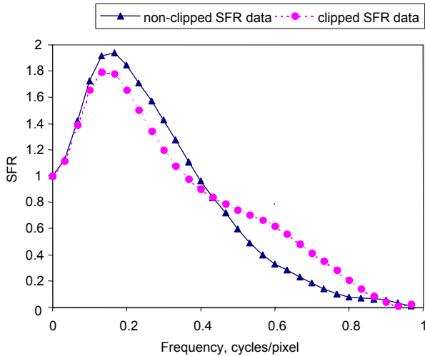
Figure 4. Measured SFR for image data with sharpening filter applied, with and without signal clipping
