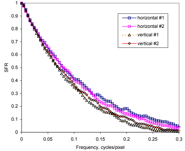
Figure 8: SFR measurements from independent edge slope estimates for the same device
