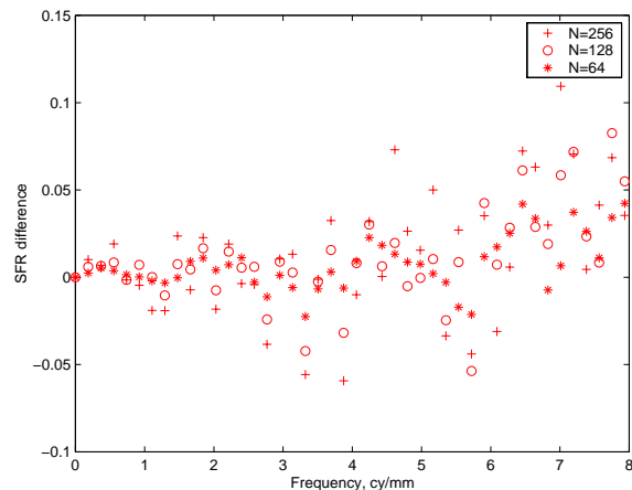
Figure 3. SFR measurement error for simulated edge with image noise and varying data lengths
