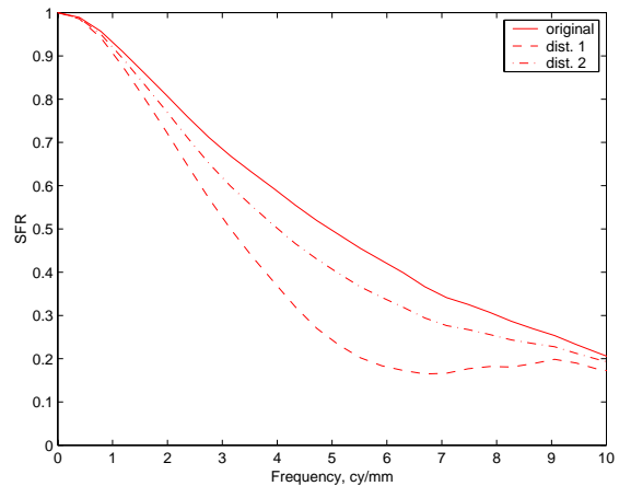
Figure 6. Measured SFR for undistorted edge and as described in Fig. 5
