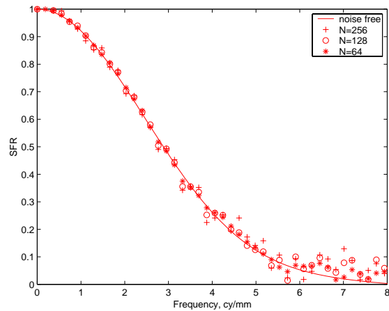
Figure 2: SFR measurements from simulated edge with image noise for varying data lengths
