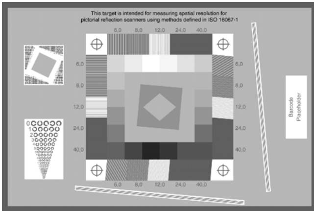
Figure 7. ISO scanner resolution target
