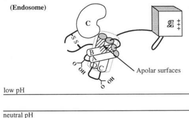
Fig. 8. The proposed structure-based mechanism of intoxication by DT shown schematically. The 3 domains of the DT molecule are labeled C (catalytic, residues 1-190), T (transmembrane, residues 191-378), and R (receptor-binding, residues 379-535). Panel 1: Proteolysis of the disulfide-linked surface loop (residues 186-201) allows the C domain to dissociate from the T and R domains when the disulfide bond between residues 186 and 201 is reduced in the cell. Three salt bridges between the C and R domains (Asp 47-His 492, Asp 97-Lys 447, Glu 148-Lys 456) are indicated by the symbols - and +, representing acidic and basic residues, respectively. Panel 2: Receptor binding by a \beta -hairpin loop (residues 514-525) shown protruding from the surface of the R domain. Panel 3: Open monomer formation triggered by low pH. Protonation of acidic residues in the C domain probably weakens 3 salt bridges between the C and R domains. Four potential transmembrane helices are represented as cylinders and labeled A (residues 269-289), B (residues 301-321), C (residues 328-348), and D (residues 351-371). The open monomer exposes apolar surfaces on helices B and D, indicated as striped patches. Acidic residues (Asp 290, Glu 292, Asp 295, Glu 298, Glu 349, and Asp 352) in the loops between helices A and B and helices C and D are represented as protonated carboxylate groups. Panel 4: The molecular mechanism of translocation remains obscure (see text). Panel 5: The toxic reaction involves the sequential binding of substrates. NAD binds first and may cause a conformational change in a loop covering the active-site cleft (residues 34-52), which allows EF-2 to bind. After the transfer of ADP-ribose to EF-2 (inactivating EF-2), the C domain undergoes subsequent rounds of catalysis.
