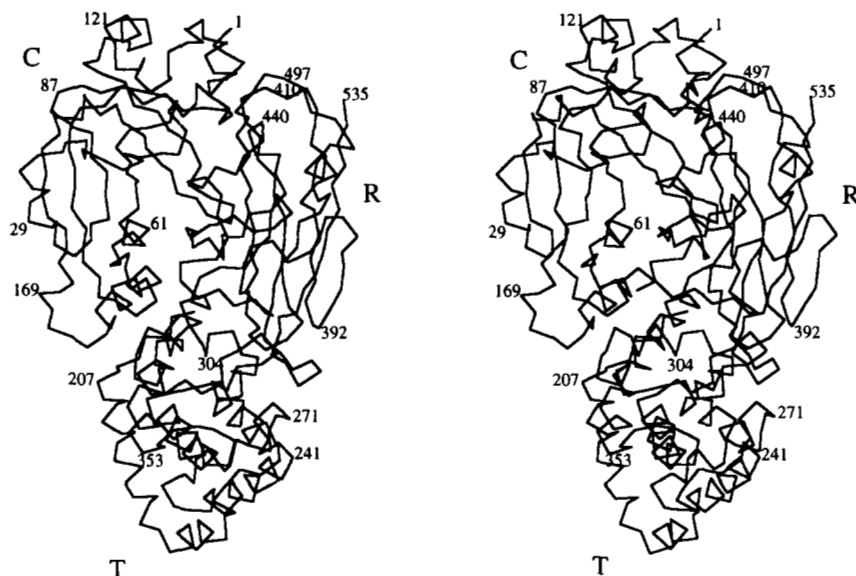
Fig. 2. Stereo figure of the C \alpha atoms of monomeric DT. Residues 188–199, in a disordered loop connecting the C and T domains, are not included in the model. The domains are indicated by the letters C (catalytic), T (transmembrane), and R (receptor-binding). Some residues are labeled for identification.
