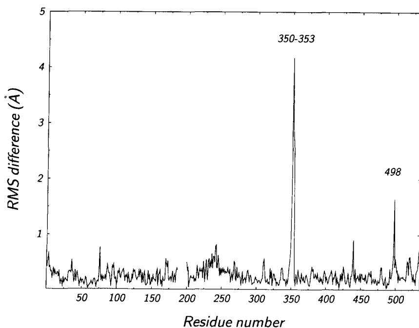
Fig. 1. Comparison of the 2 monomers in the asymmetric unit of monomeric DT crystals. RMS differences between C\alpha atoms are plotted against residue number and residues with RMS differences >1 Å are labeled. Excluding residues 350–353, which are modeled differently in the 2 monomers, and residue 498 in a surface loop, the overall RMS difference is 0.3 Å. RMS differences were calculated using the program OVERLAY (Kabsch, 1978) with a 2-Å cutoff.
