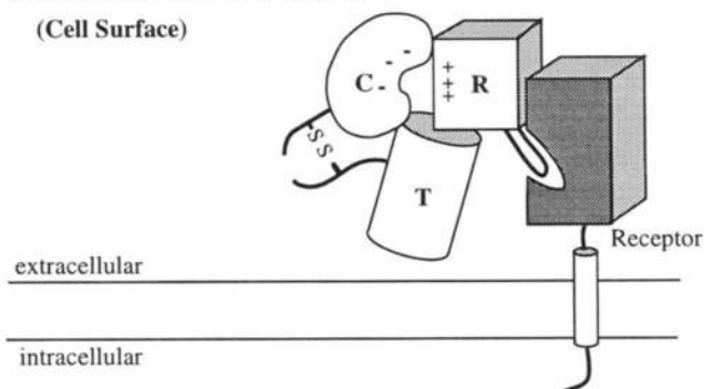
Fig. 8. The proposed structure-based mechanism of intoxication by DT shown schematically. The 3 domains of the DT molecule are labeled C (catalytic, residues 1-190), T (transmembrane, residues 191-378), and R (receptor-binding, residues 379-535). Panel 1: Proteolysis of the disulfide-linked surface loop (residues 186-201) allows the C domain to dissociate from the T and R domains when the disulfide bond between residues 186 and 201 is reduced in the cell. Three salt bridges between the C and R domains (Asp 47-His 492, Asp 97-Lys 447, Glu 148-Lys 456) are indicated by the symbols - and +, representing acidic and basic residues, respectively. Panel 2: Receptor binding by a \beta -hairpin loop (residues 514-525) shown protruding from the surface of the R domain. Panel 3: Open monomer formation triggered by low pH. Protonation of acidic residues in the C domain probably weakens 3 salt bridges between the C and R domains. Four potential transmembrane helices are represented as cylinders and labeled A (residues 269-289), B (residues 301-321), C (residues 328-348), and D (residues 351-371). The open monomer exposes apolar surfaces on helices B and D, indicated as striped patches. Acidic residues (Asp 290, Glu 292, Asp 295, Glu 298, Glu 349, and Asp 352) in the loops between helices A and B and helices C and D are represented as protonated carboxylate groups. Panel 4: The molecular mechanism of translocation remains obscure (see text). Panel 5: The toxic reaction involves the sequential binding of substrates. NAD binds first and may cause a conformational change in a loop covering the active-site cleft (residues 34-52), which allows EF-2 to bind. After the transfer of ADP-ribose to EF-2 (inactivating EF-2), the C domain undergoes subsequent rounds of catalysis.
